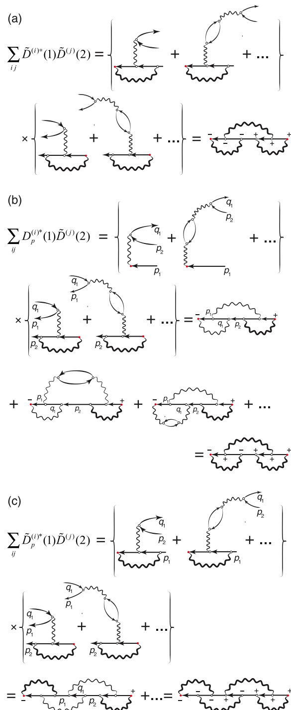
FIG. 14. (Color online) There are four extra diagrams that correct the self-energy with three \pm g lines ( \Sigma_3 ). They have (a) \tilde{D}^*(1)\tilde{D}(2) , (b) D_p^*(1)\tilde{D}(2) , \tilde{D}_p^*(1)D(2) [similar to diagram (b) and thus not shown], and (c) \tilde{D}_p^*(1)\tilde{D}(2) structures. Subscript P denotes a diagram with permuted p indices.
