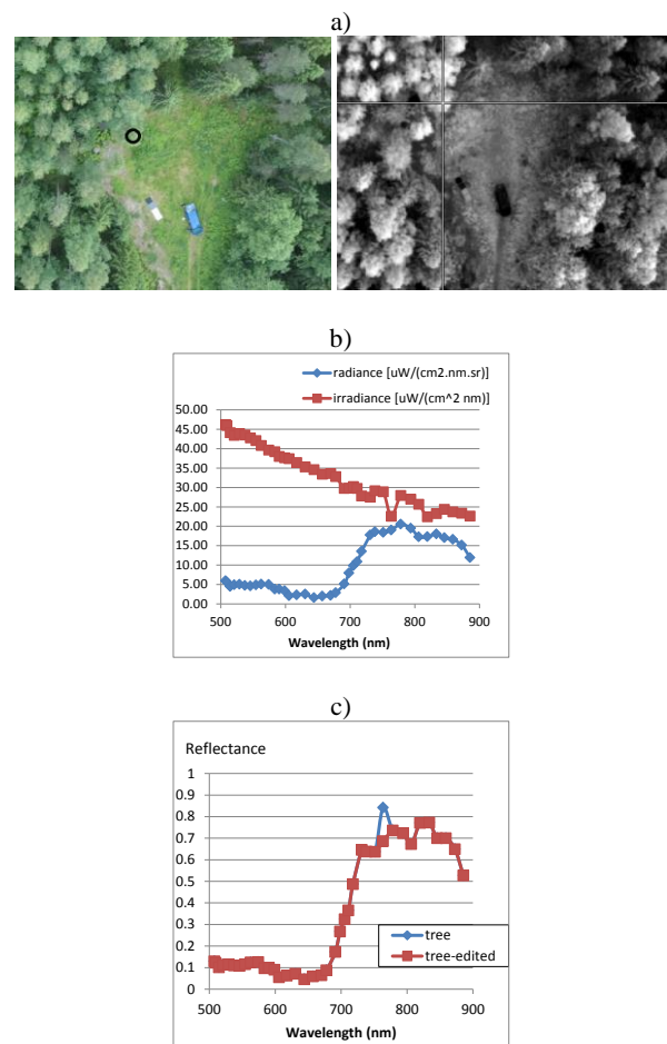
Figure 6. An example of reflectance measurement on a tree top. a) RGB and FPI image ( \lambda_0=764 \text{ nm} ). b) Tree top radiance spectrum and the irradiance spectrum during the exposure. c) Reflectance of the tree top; tree: full spectra; tree-edited: without the problematic observation at \lambda_0=764 \text{ nm} .
