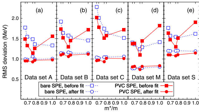
FIG. 5 (color online). Open (full) symbols: rms deviations between the bare (PVC-corrected) SPEs and empirical data of sets A (a), B (b), C (c), M (d), and S (e) (see text). Results obtained for the five studied Skyrme EDFs (squares), and for the corresponding refitted parametrizations (circles), are shown in the function of the effective mass corresponding to the original Skyrme EDF parametrizations.
