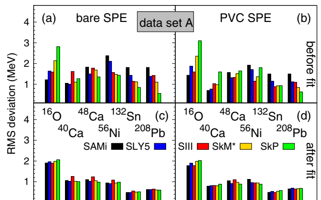
FIG. 4 (color online). Left: (a) and (c) [right (b) and (d)] panels: rms deviations between the bare [PVC-corrected] SPEs and empirical data of set A. Upper: (a) and (b) and lower: (c) and (d) panels show results obtained for standard Skyrme EDFs and for refitted parametrizations, respectively. In all cases, partial contributions obtained in six doubly magic nuclei are shown.
