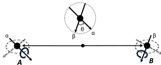
Figure 1. Entanglement paradigm. Schematic representation of two spin-1/2 particles, e.g., electrons, in the singlet state (represented by \langle \uparrow \otimes \downarrow - \downarrow \otimes \uparrow \rangle in quantum-mechanical notation) running away from each other. The directions \alpha and \beta are detector settings for spin measurements (in our language, inputs). The measured spins A and B (outputs) in these directions are shown by rotation arrows: one direction of rotation (say, clockwise) represents “spin-up” = +1 in one particle and “spin-down” = -1 in the other. By the quantum theory, for any \alpha, \beta , \Pr[A = +1, B = +1] = 1/2 \cos^2 \theta/2 (equivalently, expected value of AB is \cos \theta ). The two measurements are made simultaneously (in some inertial frame of reference). doi:10.1371/journal.pone.0061712.g001
