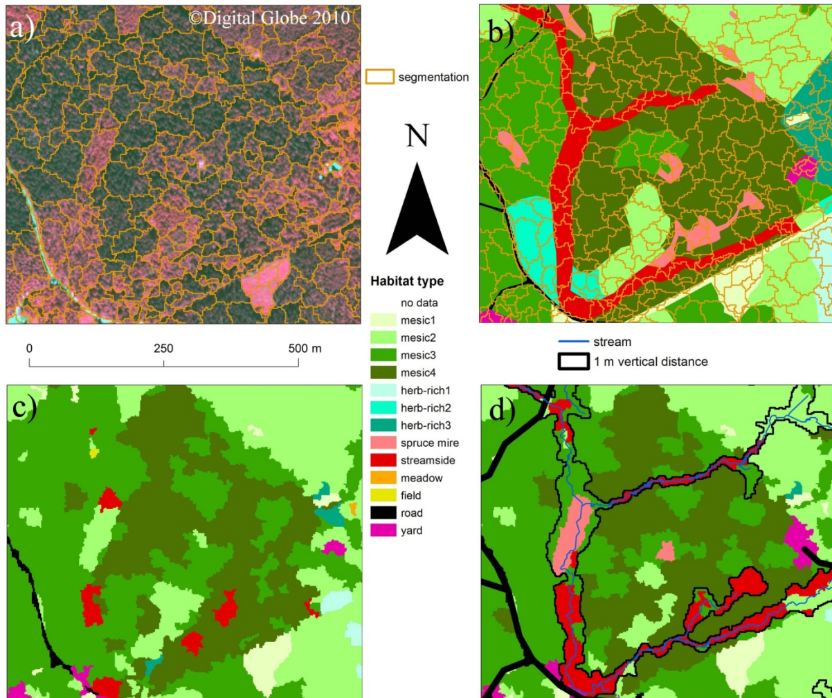
Figure 3. Classification example inside easternmost sub-area. a) WV-2 imagery (Red: band 7, G: band 5, B: band 3) shown with segmentation boundaries. b) Field work reference polygons shown with segmentation boundaries. c) Classification output with 100 features selected with Boruta. d) Classification output with data split and 100 features selected by Boruta and ancillary data. Also mapped stream network and 1 m vertical distance to the nearest stream are shown.
