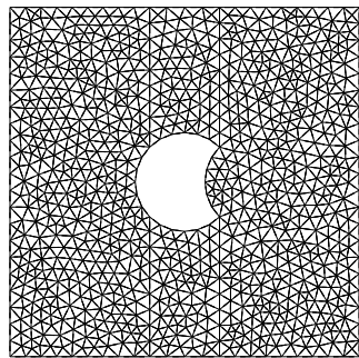
(a) Mesh for the method with shifted-Laplacian preconditioning.
