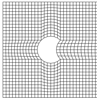
(b) Mesh for the control method.
