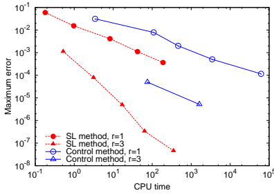
Figure 1. Errors with respect to CPU time (in seconds). On each line, mesh step size is divided by two, consecutively, and angular frequency \omega = 2\pi is kept constant.
