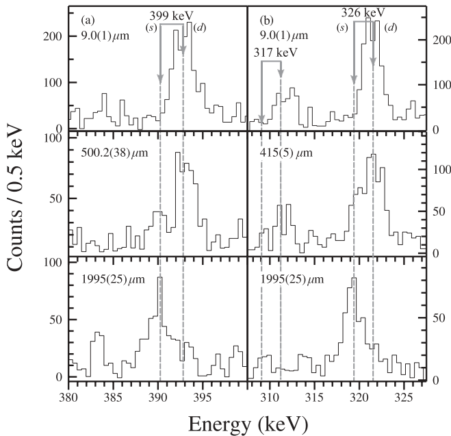
FIG. 4. Example of recoil-gated \gamma - \gamma coincidence spectra for three target-to-degrader distances for panel (a), the 399- and panel (b), the 326-keV transitions in ^{109}\text{Te} . The 326- and 399-keV peaks were measured after a summation of gates placed on the higher-lying 695- and 609-keV transitions. The fully Doppler-shifted, (s) and degraded, (d) components of each transition have been highlighted. Panel (b) also highlights the expected positions of the fully Doppler shifted and degraded components of the 317-keV \gamma ray. No Doppler correction has been applied to the spectra.
