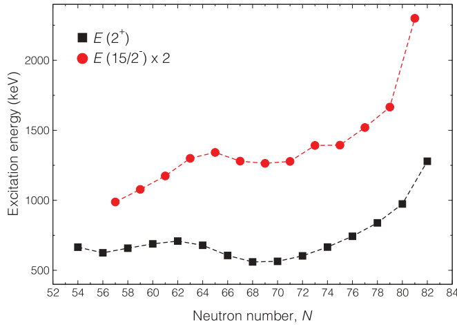
FIG. 6. (Color online) Excitation energies of the first excited states in the ground-state bands of the even-mass tellurium isotopes (squares) and the \nu h_{11/2} bands (circles) of the odd-mass tellurium isotopes (relative to the 11/2^- band-head). Energies in the odd-mass isotopes have been multiplied by a factor of two to separate them from those of the even-mass isotopes. Data were taken from Refs. [5–8,37–43].
