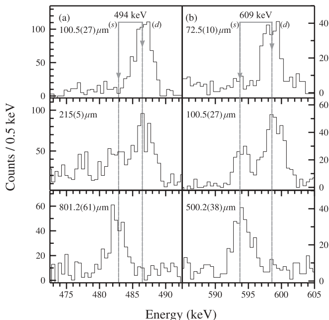
FIG. 2. Example of recoil-gated \gamma - \gamma coincidence spectra for three target-to-degrader distances for panel (a), the 494- and panel (b), the 609-keV transitions in ^{109}\text{Te} . The 494-keV gated spectra were produced from a gate on the higher-lying 695-keV \gamma ray. The 609-keV gated spectra were collected from an energy gate on the higher-lying 890-keV transition. The fully Doppler-shifted, (s) and degraded, (d) components of each transition have been highlighted. No Doppler correction has been applied to the spectra.
