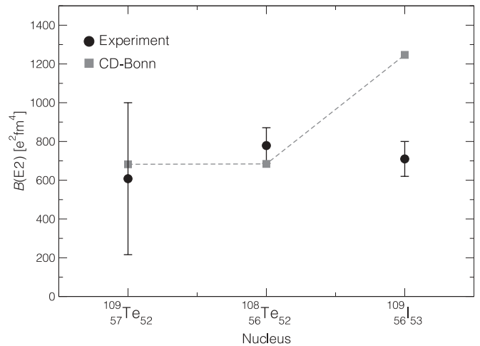
FIG. 9. Comparison of theoretical B(E2) values, determined from shell-model calculations, with the experimentally measured values for the ground-state transitions in ^{109}\text{Te} , ^{108}\text{Te} and ^{109}\text{I} . The theoretical values have been calculated with standard proton and neutron effective charges of e_p = 1.5e and e_n = 0.5e , respectively.
