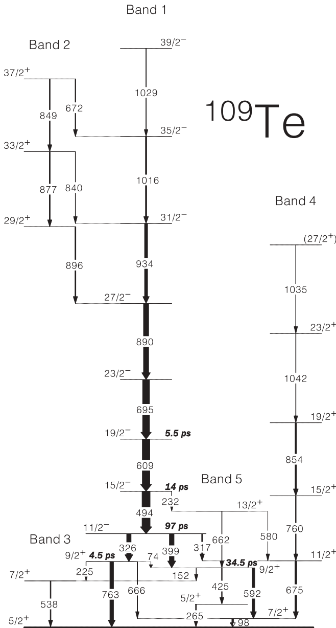
FIG. 1. Partial level scheme of ^{109}\text{Te} showing the transitions observed in this work. The transition energies are given in keV with the relative intensities given by the width of the arrows. The intensities were determined from \gamma - \gamma coincidence data collected at the shortest target-to-degrader distance, 9\ \mu\text{m} where the majority of transitions are observed to reside in the Doppler-degraded component of the photopeak. The lifetimes of the states measured in this work are shown in bold text.
