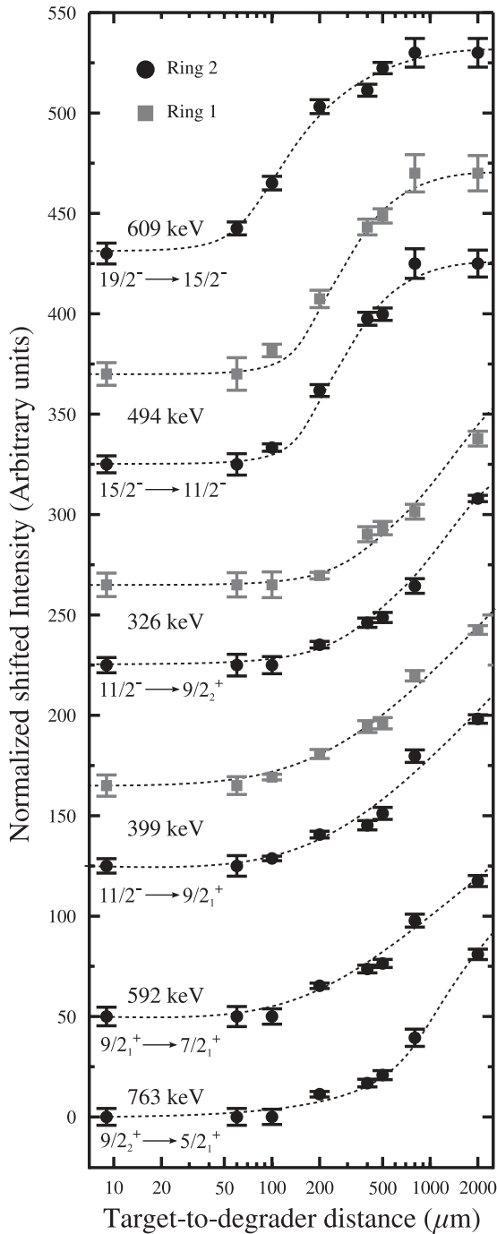
FIG. 3. Normalized shifted intensities for the transitions in ^{109}\text{Te} measured in this work. Square data points correspond to measurements from Ring 1 and circle data points measurements from Ring 2. The errors are derived solely from the statistical uncertainty in the intensity measurement of the two components of each photopeak. The dashed curves are drawn to guide the eye.
