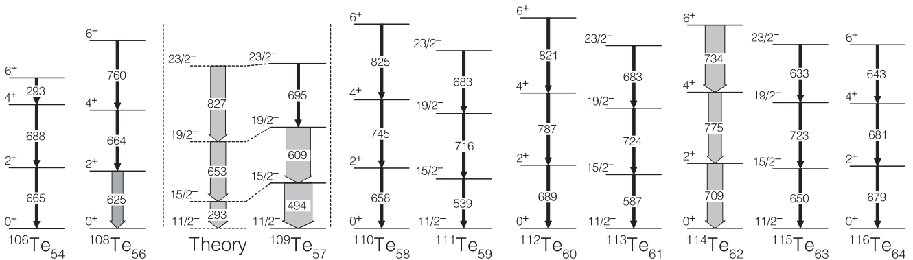
FIG. 7. Experimental excitation energies in the \nu h_{11/2} bands of odd-mass tellurium nuclei for N < 63 compared with their even-even ground-state counterparts. Theoretical CD-Bonn calculations for ^{109}\text{Te} are also shown to the left of the experimental measurements. For states with experimentally measured B(E2) values, the width of the shaded arrows denotes the strength of the decay normalised to the 15/2^- \rightarrow 11/2^- B(E2) value in ^{109}\text{Te} . It should be noted that the ordering of the \gamma -ray transitions in ^{106}\text{Te} is tentative. The data for each of the tellurium isotopes are taken from [5–8,44–48]. States built upon the \nu h_{11/2} level in ^{107}\text{Te} are yet to be observed.
