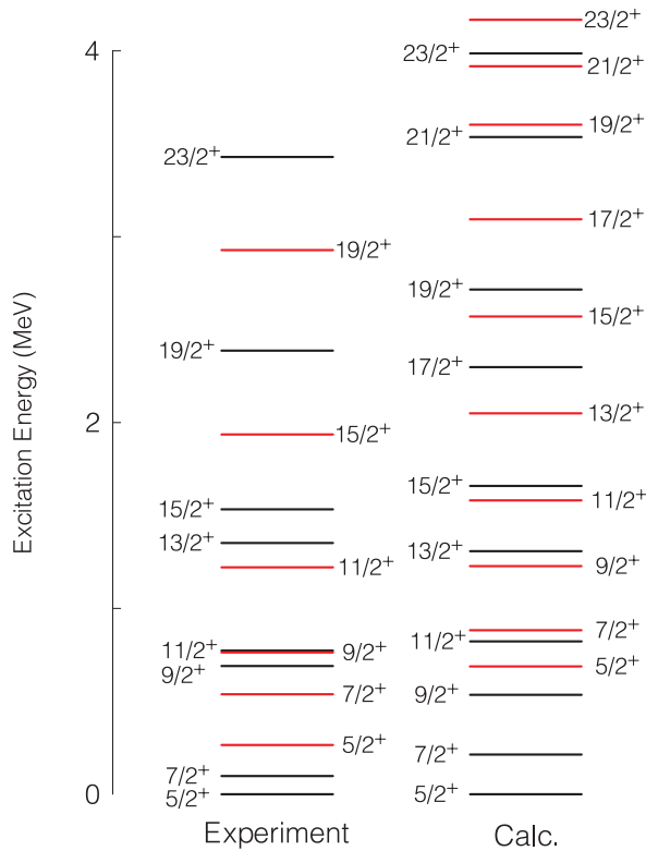
FIG. 8. (Color online) Experimental and theoretical excitation energies for the low-lying positive-parity states in ^{109}\text{Te} . Both the first and second (red) excited states for a given spin are shown.
