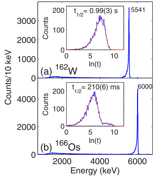
FIG. 1. (Color online) (a) Spectrum of the recorded \alpha -decay energies from ^{162}\text{W} ground-state decays produced by requiring a preceding \alpha decay from the mother nucleus ^{166}\text{Os} and a subsequent \alpha decay from the granddaughter nucleus ^{158}\text{Hf} in the same pixel in the DSSSDs. In order to minimize the influence from random correlations, decay chains were selected for analysis by applying maximum correlation times between successive events. The maximum correlation times between recoil implantation and ^{166}\text{Os}\alpha decay, and between ^{162}\text{W}\alpha decay and ^{158}\text{Hf}\alpha decay, were set to 0.6 and 9 s, respectively. The inset shows the distribution of time differences between mother nucleus ^{166}\text{Os}\alpha decay and the daughter ^{162}\text{W}\alpha decay. A 990(30)-ms half-life is extracted for ^{162}\text{W} as described in the text. (b) Spectrum showing the recorded \alpha -decay energies of ^{166}\text{Os} produced by requiring an additional \alpha decay from the daughter nucleus ^{162}\text{W} and the \alpha decay from the granddaughter nucleus ^{158}\text{Hf} in the same pixel in the DSSSDs. The maximum correlation times between ^{166}\text{Os}\alpha decay and ^{162}\text{W}\alpha decay, and between ^{162}\text{W}\alpha decay and ^{158}\text{Hf}\alpha decay, were set to 6 and 9 s, respectively. The inset shows the distribution of time differences between implanted recoils and ^{166}\text{Os}\alpha decays. A 210(6)-ms half-life is extracted for the ground state of ^{166}\text{Os} .
