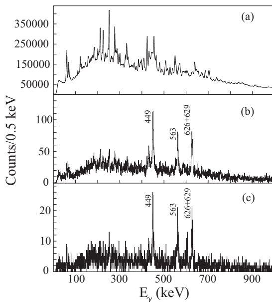
FIG. 2. (a) \gamma -ray spectrum of recoil-tagged singles. (b) ^{162}\text{W} mother-daughter correlated \alpha -decay-tagged \gamma -ray singles. The maximum correlation time between recoils and mother nucleus ( ^{162}\text{W} ) \alpha decays and subsequent daughter nucleus ( ^{158}\text{Hf} ) \alpha decays are 3 and 6 s, respectively. The unmarked peaks are the \gamma -ray transitions from the strong populated channels. (c) As in panel (b) with the additional requirement of granddaughter ^{154}\text{Yb} \alpha decay correlated within 1.2 s in the same pixel of the DSSSDs.
