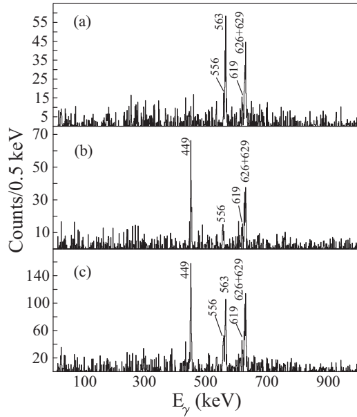
FIG. 4. Background-subtracted spectra of \gamma rays tagged by the ground-state \alpha decay of ^{162}\text{W} and detected in prompt coincidence with the (a) 449-keV \gamma ray, (b) 563-keV \gamma ray, and (c) 449-, 563-, 626-, or 629-keV \gamma rays.
