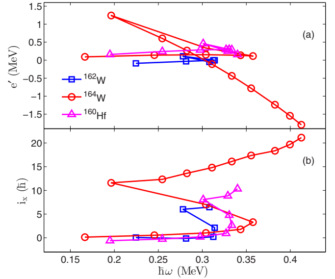
FIG. 7. (Color online) (a) Experimental Routhians and (b) aligned angular momenta for the ground-state bands in ^{162}\text{W} (present work), ^{164}\text{W} [22], and ^{160}\text{Hf} [26]. A rotational reference configuration has been subtracted using the Harris parameters \mathcal{J}_0 = 1\hbar^2/\text{MeV} and \mathcal{J}_1 = 196\hbar^4/\text{MeV}^3 , for ^{162}\text{W} , while those for ^{164}\text{W} and ^{160}\text{Hf} are taken from Refs. [22,26].
