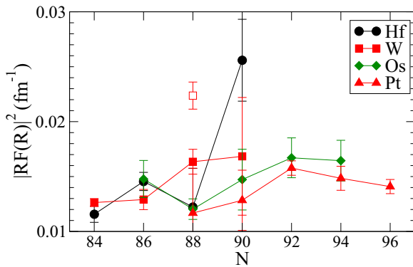
FIG. 9. (Color online) \alpha -formation probabilities |\text{RF}(\text{R})|^2 calculated from experimental \alpha -decay partial half-lives as a function of the neutron number, N , for the \alpha decays of even-even Hf, W, Os, and Pt isotopes. The experimental data represented by solid symbols are from NNDC [32]. Our new data for ^{162}\text{W} is shown as the open symbol.
