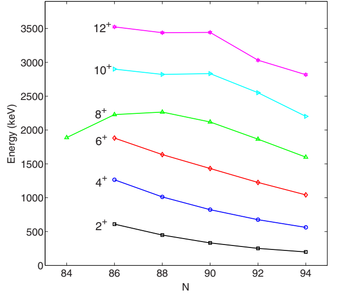
FIG. 5. (Color online) Yrast level energies in the most neutron-deficient even- N tungsten isotopes with N = 84 – 94 [20–24].
