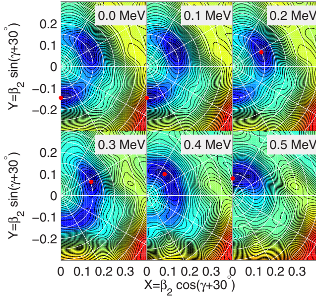
FIG. 6. (Color online) The TRS calculations for ^{162}\text{W} at \hbar\omega = 0.0 to 0.5 MeV. The energy difference between successive contour curves is 200 keV. Red (gray) dots indicate the positions of the minima in the surfaces.
