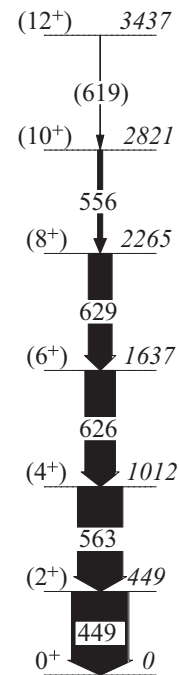
FIG. 3. Proposed level scheme for ^{162}\text{W} . Energies are given in keV. Spin and parity assignments are tentative. The widths of the arrows indicate the relative transition intensities.
