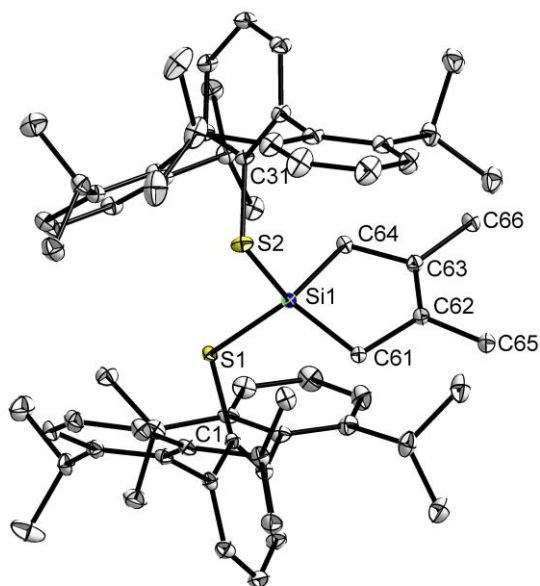
Figure 3. Thermal ellipsoid plot (30 %) of the molecular structure of 3 . Hydrogen atoms and co-crystallized toluene molecules are not shown. Selected bond distances [Å] and angles [°]: Si1–C61 1.8831(12), Si1–C64 1.8810(13); C61–C62 1.5249(17), C64–C63 1.5252(17), C62–C63 1.3340(19), C62–C65 1.5059(18), C63–C66 1.5036(18), Si1–S1 2.1495(4), Si1–S2 2.1456(5), S1–C1 1.7985(12), S2–C31 1.7885(13); C61–Si1–C64 96.08(5), Si1–C64–C63 102.31(8), Si1–C61–C62 102.47(8), C64–C63–C62 118.93(11), C61–C62–C63 118.49(11), S1–Si1–S2 106.337(18), C1–S1–Si1 106.44(4), C31–S2–Si1 106.70(4), S1–Si1–C61 114.89(4), S2–Si1–C64 110.93(4).
