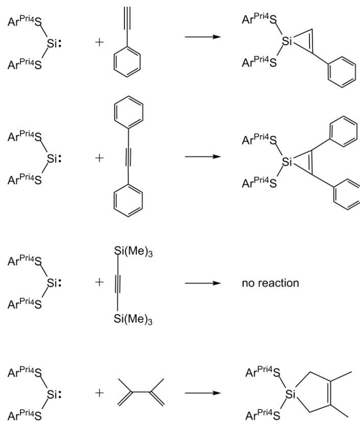
Scheme 1. Reactions of \text{Si}(\text{SAr}^{i\text{Pr}_4})_2 with phenylacetylene, diphenylacetylene, bis(trimethylsilyl)acetylene, and 2,3-dimethyl-butadiene.
