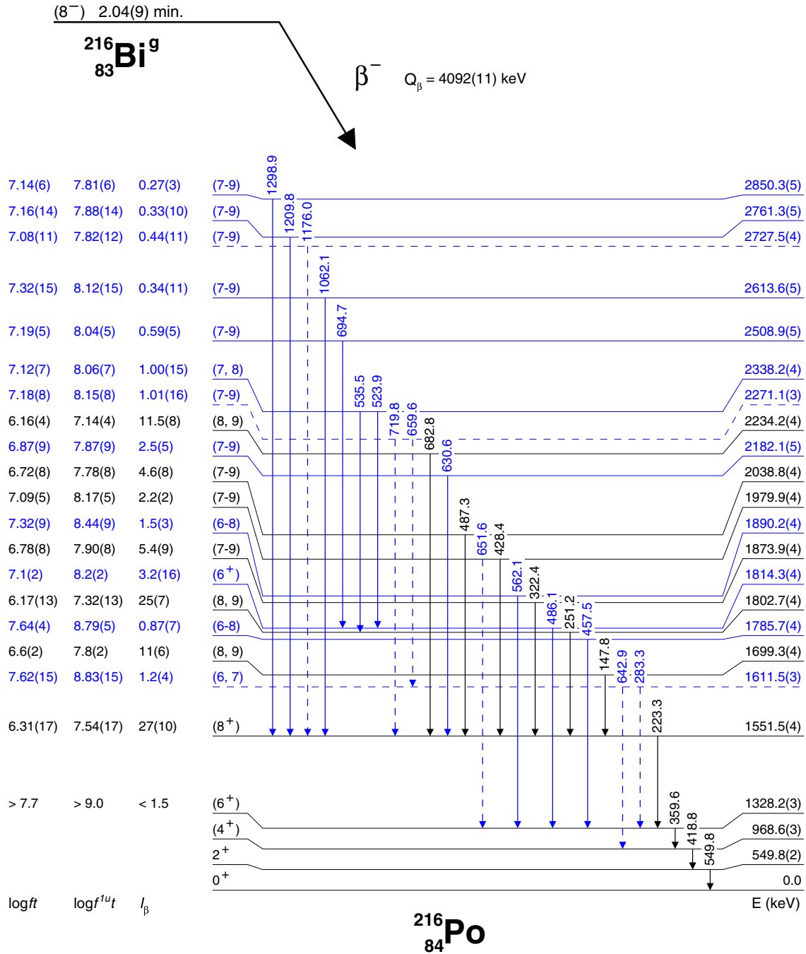
FIG. 2. The decay scheme with levels in 216 Po populated by the \beta^- decay of 216 Bi g . The new transitions and levels from the present study are highlighted in blue, while those in black font were reported in Refs. [4,5]. The half-life of 216 Bi g , \beta -decay feeding intensities and \log(ft) , \log(f^{1u}t) values are from this work. All spin and parity assignments are from this work, with an exception of the yrast levels in 216 Po up to the (8 + ) state, which were taken from Ref. [4]. The Q_\beta value was taken from AME 2020 [35]. For display purposes, the levels up to the (6 + ) state are spaced evenly. Dashed lines denote tentatively placed transitions and levels.
