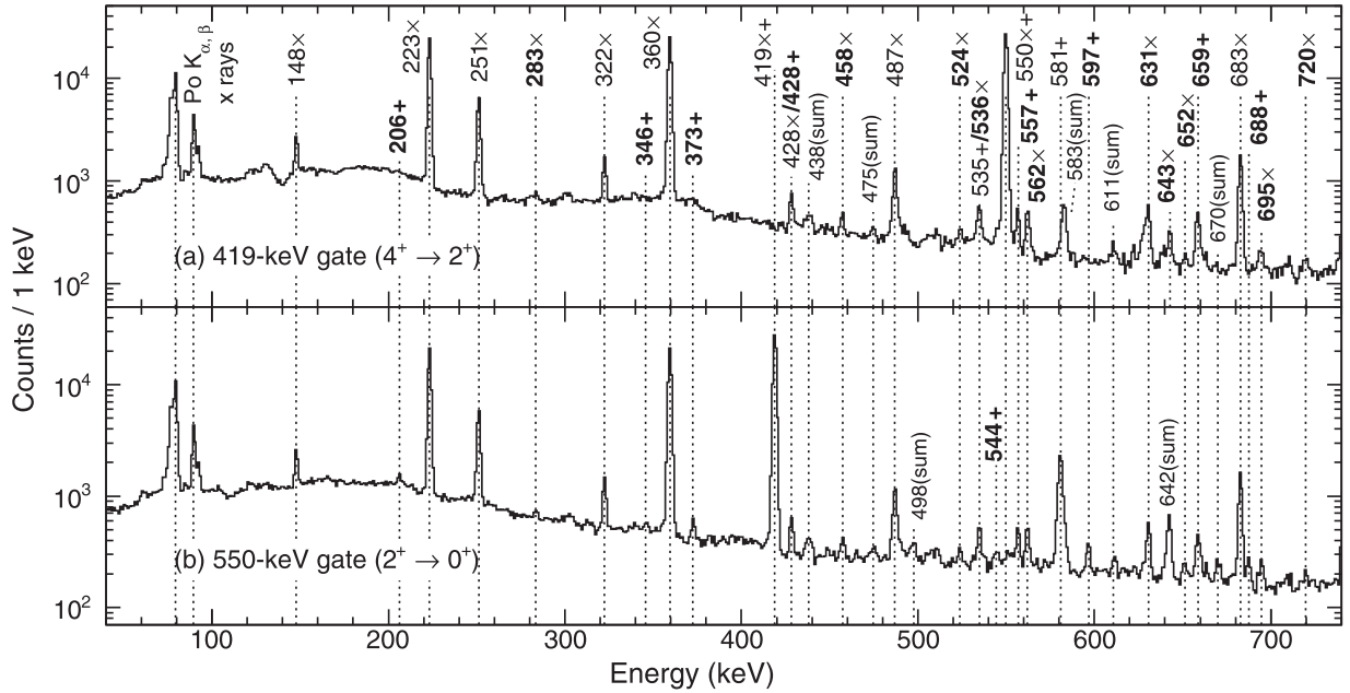
FIG. 5. The low-energy part of the background-subtracted spectra of \gamma rays in coincidence with (a) the 418.8-keV ( 4^+ \rightarrow 2^+ ) and (b) the 549.8-keV 2^+ \rightarrow 0^+ transition. The peaks marked with ( \times ) and ( + ) labels follow the \beta^- decays of ^{216}\text{Bi}^g and ^{216}\text{Bi}^m , respectively, transitions with labels in bold are new. Peaks marked with “(sum)” are caused by summing of transitions in cascades, they are listed in Table II in the Supplemental Material [15].
