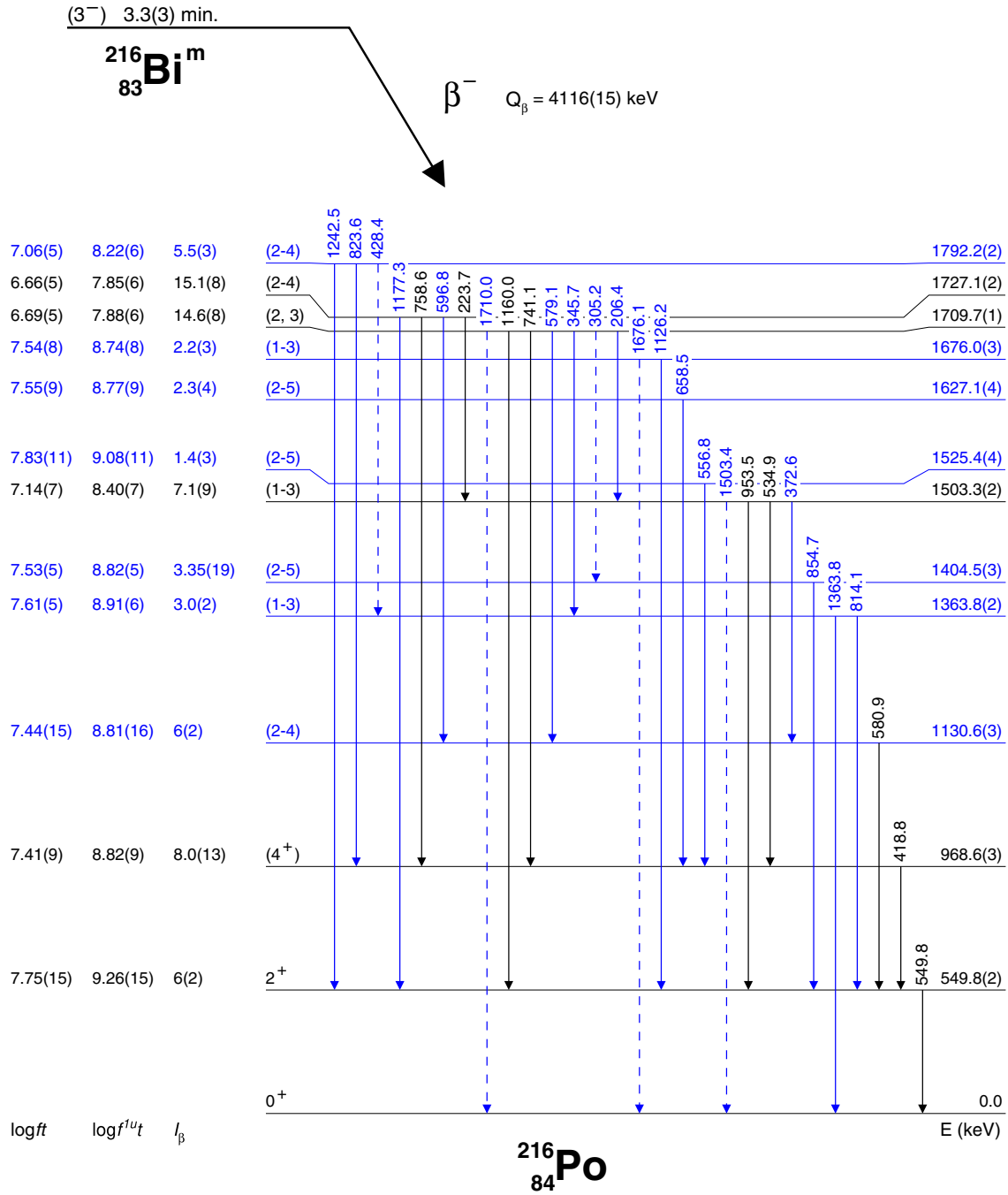
FIG. 7. The first part of the decay scheme with levels in ^{216}\text{Po} populated by the \beta^- decay of ^{216}\text{Bi}^m . The new transitions and levels from the present study are highlighted in blue, while those in black font were reported in Ref. [5]. The half-life of ^{216}\text{Bi}^m , \beta -decay feeding intensities and \log(ft) , \log(f^{1/ut}) values are from this work. All spin and parity assignments are from this work, with an exception of the yrast levels in ^{216}\text{Po} up to the (4 + ) state, which were taken from Ref. [4]. The Q_\beta value was calculated as the difference between the atomic mass excesses of ^{216}\text{Bi}^m and ^{216}\text{Po} taken from NUBASE [10]. For display purposes, the levels up to the 1130.6-keV state are spaced evenly. Dashed lines denote tentative transitions.
