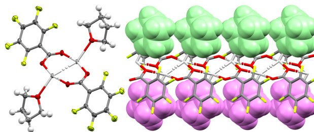
Fig. 6 A dimeric subunit of 1 ·THF (left; thermal ellipsoids at 50% probability) and the alternating axial coordination of the THF adducts in a 1D chain of eight molecules of 1 ·THF (right) above and below the plane (block coloured green and purple, respectively) of the polymeric chain of dimeric subunits of 1 .
