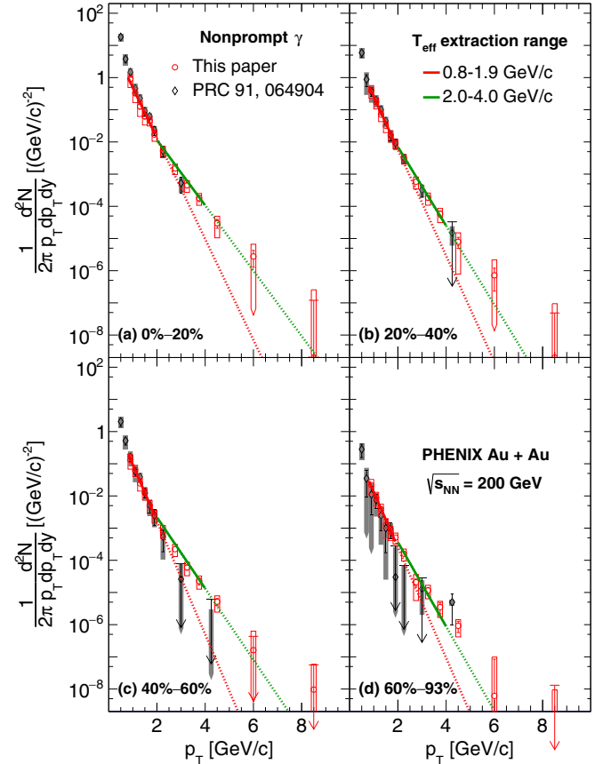
FIG. 16. Nonprompt direct-photon yield as a function of conversion photon p_T in (a) 0%–20%, (b) 20%–40%, (c) 40%–60%, and (d) 60%–93% centrality bins are compared to results from previous PHENIX publications (see Ref. [6]).
