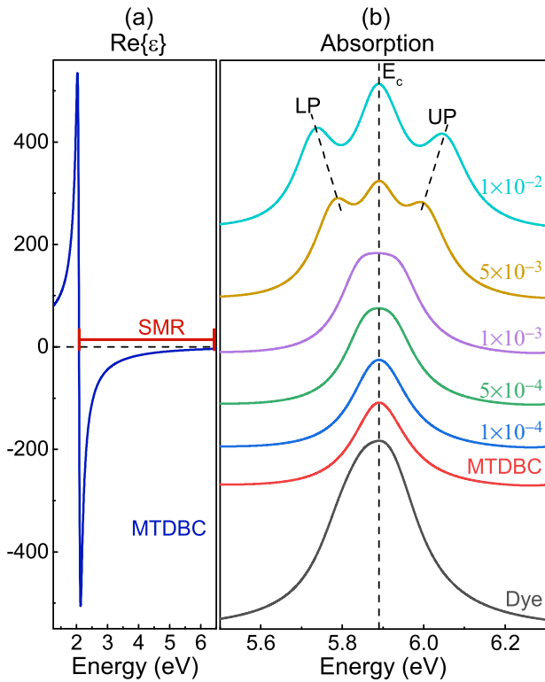
FIG. 3. (a) Real part of the dielectric function [ \text{Re}\{\epsilon(\omega)\} ] of MTDBC as a function of energy. The surface mode region (SMR)—i.e., the spectral range where \text{Re}\{\epsilon(\omega)\} < 0 , and thus, the SE modes are supported—is marked for MTDBC. (b) Absorption spectra of generic dye shell (black), MTDBC core (red), and the core-shell coupled system for different values of f_{\text{dye}} (0.0001, 0.0005, 0.001, 0.005, and 0.01). The spectra are vertically shifted for clarity. The absorption of the dye shell is spectrally tuned to match the SE mode of the MTDBC core, i.e., E_0 = E_c = 5.9 eV (vertical dashed line). The lower polariton (LP) and upper polariton (UP) branches are shown by the tilted black dashed lines. In the figure, absorption means absorption efficiency, i.e., absorption cross-sections normalized by geometrical cross-section.
