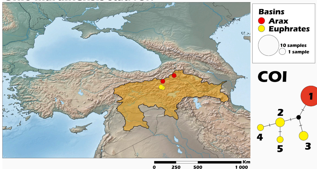
Fig. 13. LEFT: Distribution map of Unio mardinensis in the study area, showing its potential distribution in the main river basins in orange and outlined in black. Coloured dots represent sequenced populations. RIGHT: COI haplotype network (TCS) showing the relationships of all new and previously published Unio mardinensis sequences (Table S1). Circle size is proportional to observed haplotype frequencies, each dash indicates a nucleotide substitution. Colours represent individuals from each basin. (For interpretation of the references to colour in this figure legend, the reader is referred to the web version of this article.)
