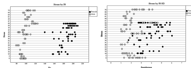
Figure 5. Scatter plot with experienced stress and F0 and F0 SD.
