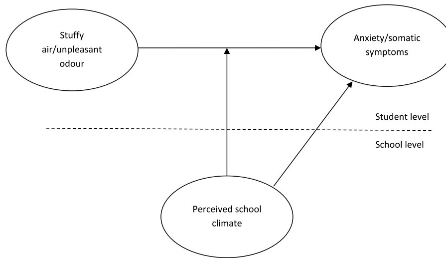
Fig. 1. Conceptual model.
