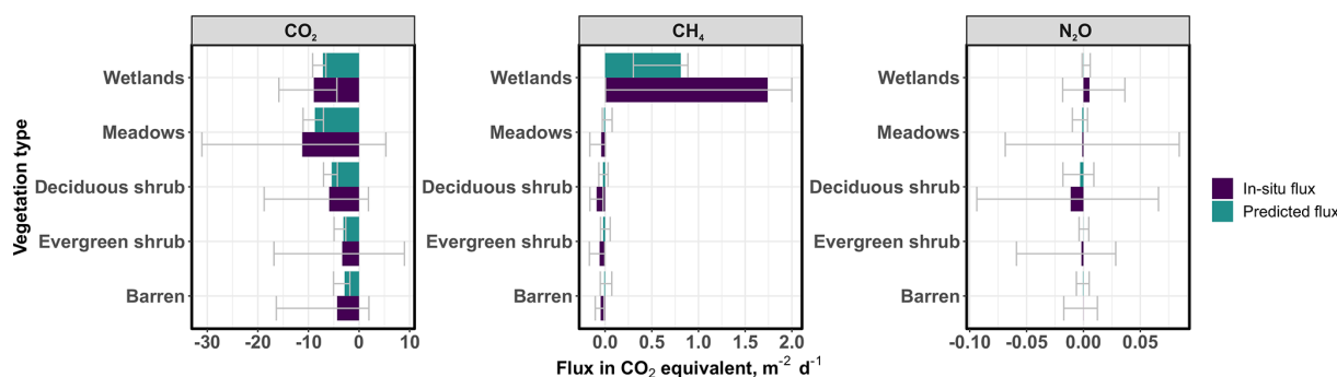
Figure 8. Growing season mean and percentile (0.025 and 0.975) GHG fluxes in CO 2 equivalents based on in situ data and upscaled flux predictions, averaged across the entire study period (only daytime variability between 08:00 and 20:00 considered) and across vegetation types. Note that the scale for the x axis is different for each gas species, and that the uncertainties in in situ versus predicted mean fluxes cannot be directly compared with each other. The uncertainty in in situ wetland CH 4 continues up to 6.7 but was cropped for visualization purposes. The same graph using the sustained GWP approach can be found in the Supplement Fig. 6 and demonstrates the potentially larger role of CH 4 fluxes over a 100-year horizon in this landscape.
