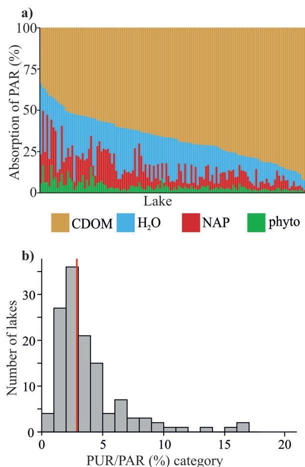
Fig. 3. The percentage of incoming PAR absorbed by (a) the four components and (b) phytoplankton in the 128 sampled lakes. In (a) the barplot shows the relative absorption of PAR by CDOM, H 2 O, NAP, and phytoplankton (phyto, i.e., PUR/PAR) in each sampled lake. In (b) the histogram shows the variation in PUR/PAR values, with the vertical red line indicating the median value.
