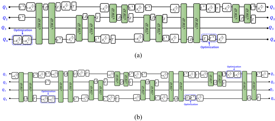
Fig. 4 Optimized decomposition of a Toffoli b Fredkin gates for QFA1
