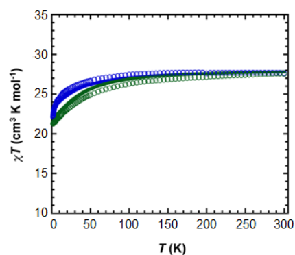
Fig. 3 Variable temperature dc magnetic susceptibility data, where \chi = M/H normalized per mole for 1-4C 6 H 6 (blue) and 2 (green) obtained under an applied field of 1000 Oe. Experimental data is denoted by circles with the solid line representing the fit.
