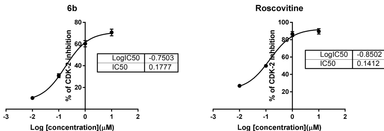
Figure 11. Dose-response curve for the CDK2 inhibition versus serial dilutions of compound 6b and roscovitine [0.01–10 \mu M].
