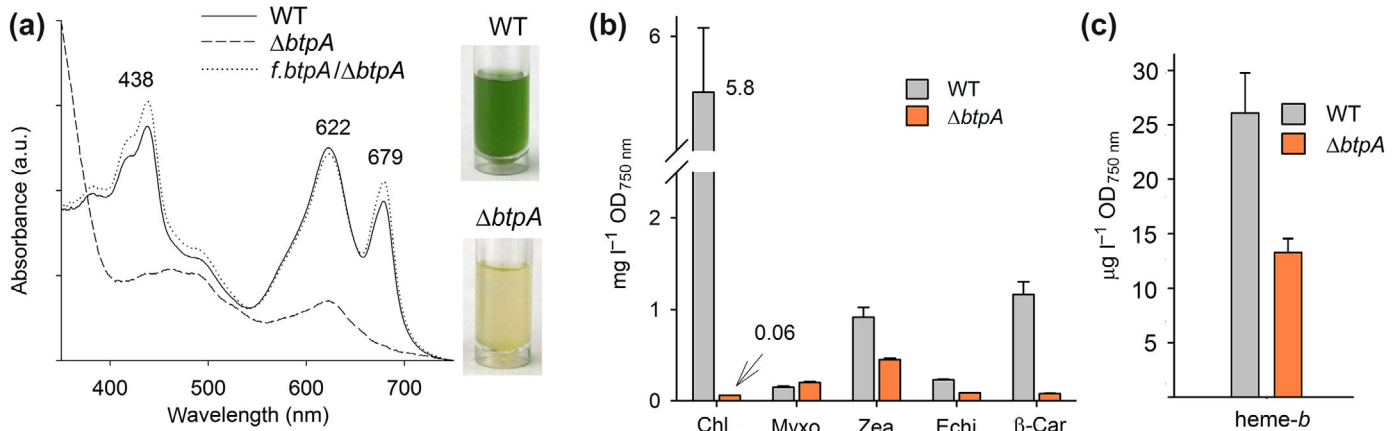
Fig. 1 Elimination of btpA gene drastically reduces chlorophyll level. (a) Whole-cell absorption spectra of wild-type (WT), btpA -null mutant ( \Delta btpA ), and f.btpA + / \Delta btpA strains grown at 5 \mu mol of photons m -2 s -1 (low light – LL) in the medium supplemented with 5 mM glucose; Chl is represented by peak at 679 nm and phycobiliproteins by peak at 622 nm. Spectra were normalized to light scattering at 750 nm. The content of photosynthetic pigments is fully restored in \Delta btpA mutant ectopically expressing FLAG-tagged BtpA ( f.BtpA ) protein. The color of cell cultures at a similar optical density is also shown. (b) Content of pigments in WT and \Delta btpA normalized to scattering at 750 nm. Pigments were extracted with methanol and quantified by high-performance liquid chromatography (HPLC); the error bars indicate the SD from the mean of biological triplicates. Echi, echinenone; Myxo, myxoxanthophyll; Zea, zeaxanthin; \beta -Car, \beta -carotene. (c) Heme- b was extracted by acetone/HCl from the same cultures as (b) and its concentration was determined by HPLC method.
