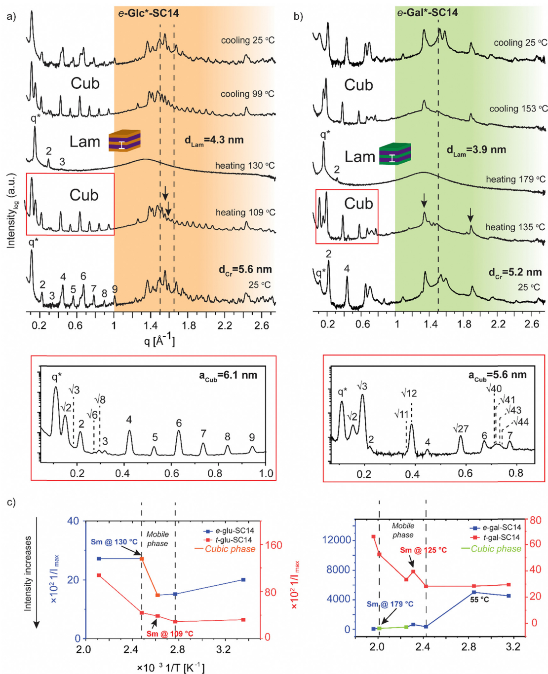
Fig. 5 Selected SWAXS profiles for (a) e-Glc*-SC14 and (b) e-Gal*-SC14 compounds. The dashed lines indicate the position of the crystalline alkyl tail peaks. The black arrows indicate possible polyol block interactions withstanding temperature increase. Colored areas represent the wide-angle regions. (c) The effect of temperature ( 1/T , between 298–463 K) on the maximum scattering intensity ( 1/I_{max} ) of the main scattering peak ( q^* ) for t-Glc*-SC14 and e-Glc*-SC14 , and t-Gal*-SC14 and e-Gal*-SC14 .
