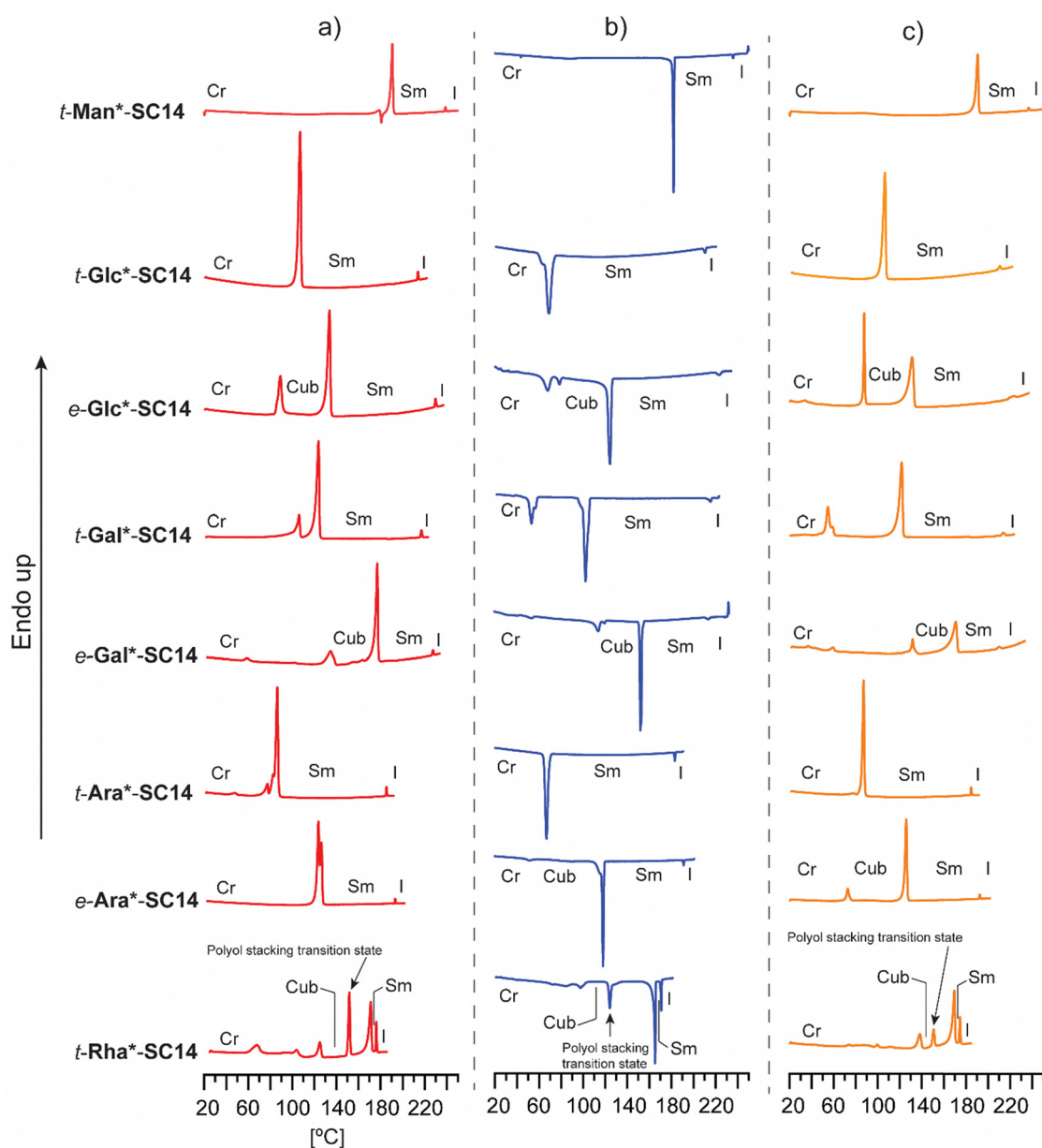
Fig. 2 Full DSC analysis with (a) heating, (b) cooling (c) and second heating traces for t-Man*-SC14 , t-Glc*-SC14 and e-Glc*-SC14 , t-Gal*-SC14 and e-Gal*-SC14 , t-Ara*-SC14 and e-Ara*-SC14 , and t-Rha*-SC14 . The identified phase transitions (Cr = crystalline, Cub = cubic, Sm = smectic and I = isotropic state) combining POM results are marked in the data.
