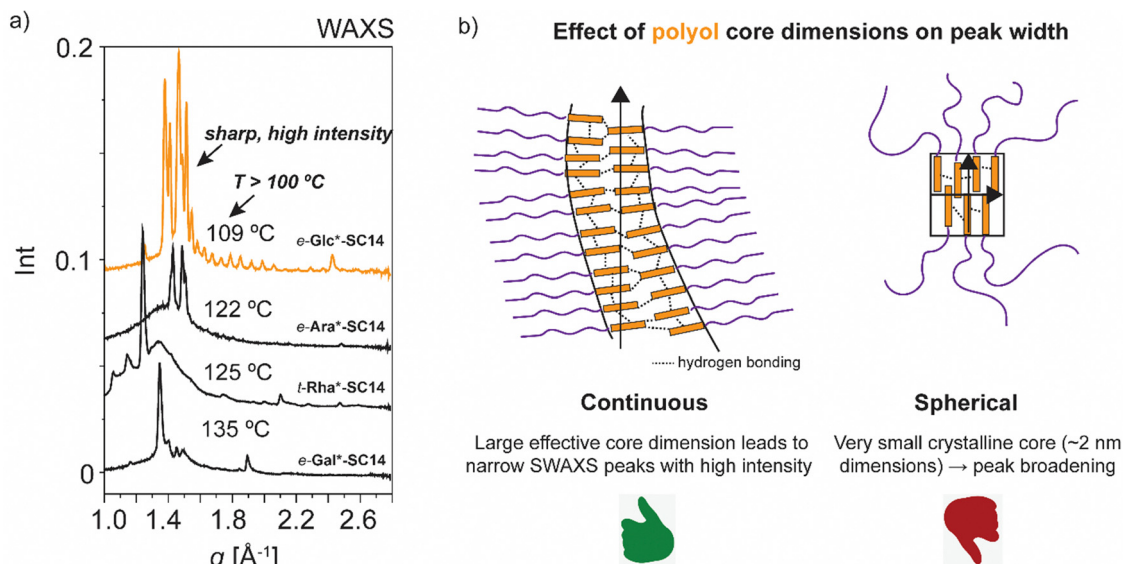
Fig. 8 (a) Selected WAXS data for e-Glc*-SC14 , e-Gal*-SC14 , e-Ara*-SC14 and t-Rha*-SC14 cubic phases upon heating. (b) Schematics describing the suggested possible cubic phase structure, favoring the continuous core structure formation using e-Glc*-SC14 as an example compound. The small crystalline domains forming a spherical cubic phase would show peak broadening in SWAXS, not seen for the compounds in question.
