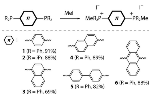
Scheme 1. Synthesis of diphosphonium iodides 1–6 .
