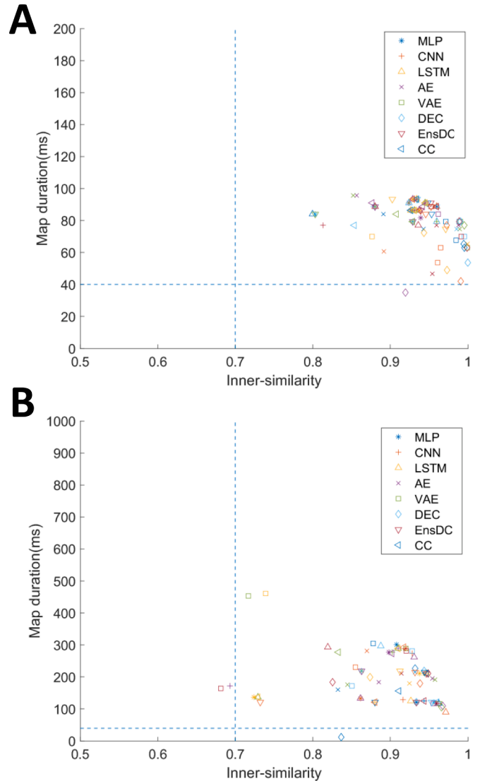
Fig. 3. Illustration of the M-N plot pre-test of the studied methods on the prepared simulated data (A) and the real data (B) with the additional noises. All the studied deep clustering designs identified cluster maps with high inner similarity (particularly noisy data resulted in lower inner similarity) from both ER data. MLP = fully connected multi-layer perceptron, CNN = one dimensional convolutional deep neural network, LSTM = long short-term memory, AE = autoencoder, VAE = variational autoencoder, DEC = deep embedded clustering, EnsDC = ensemble deep clustering, and CC = consensus clustering.
