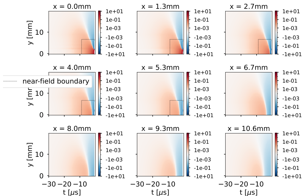
Figure 5. Induced current on a 4.4 mm pixel from a drifting electron at a given drift time and x , y position relative to the pixel, in units of electrons per 0.1 \mu\text{s} . The different calculations used for the near-field and far-field regions are described in the text in section 3.3.1 with the near-field boundary highlighted with a dotted line.
