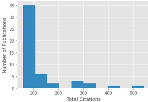
Fig. 2 Number of publications vs. total citations histogram for top-50 papers
