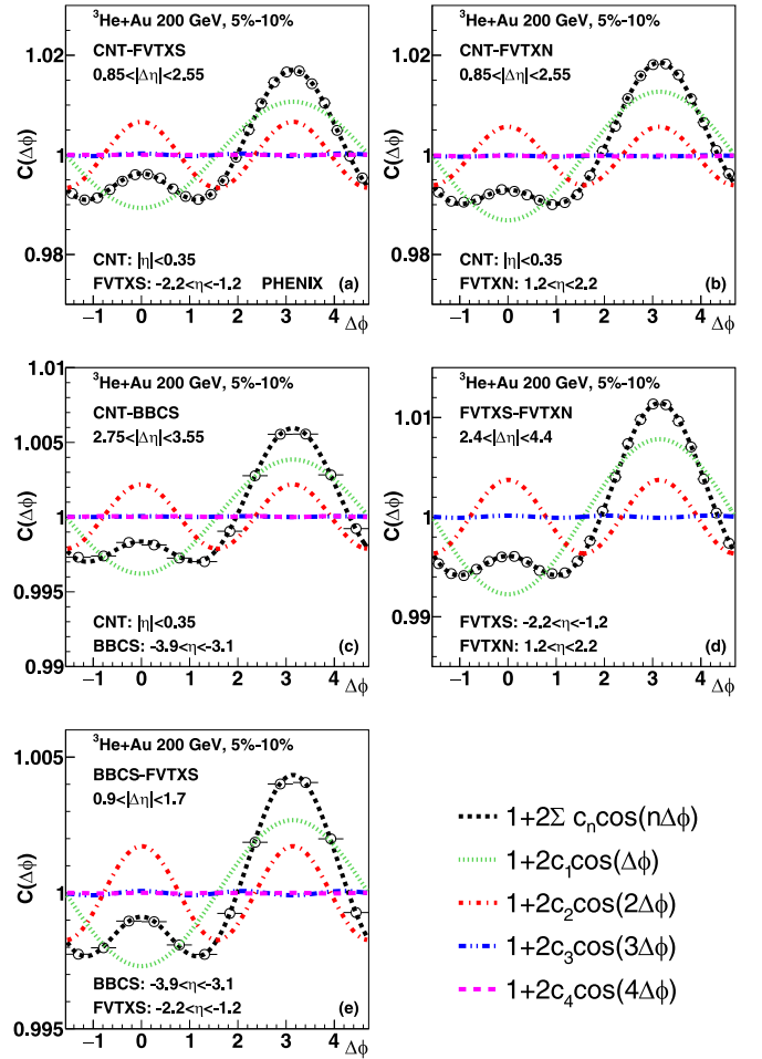
FIG. 3. Correlation functions C(\Delta\phi) in 5%–10% centrality ^3\text{He} + \text{Au} collisions at \sqrt{s_{NN}} = 200 GeV measured using (a) CNT-FVTXS, (b) CNT-FVTXN, (c) CNT-BBCS, (d) FVTXS-FVTXN, and (e) BBCS-FVTXS detector combinations. The short-dashed (black) curve shows the Fourier fit to correlation functions. The dotted (green), dash-dotted (red), dashed-double-dotted (blue), and long-dashed (magenta) curves indicate c_1 , c_2 , c_3 , and c_4 components, respectively.
