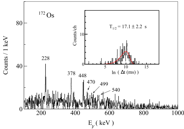
FIG. 3. Prompt RDT \gamma rays in JGII correlated with recoil implantations in the DSSDs followed by the E_\alpha = 5106 keV \alpha decay of ^{172}\text{Os} within a maximum search time of 1 minute in the same pixel. The inset shows the time difference spectrum of the correlated recoil- \alpha events within a search time of 10 minutes by gating on the prompt 228 keV \gamma rays. The fit to the logarithmic time distribution was produced using the Schmidt formula [22] indicated by the red line.
