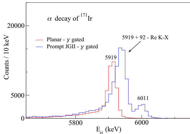
FIG. 8. Energy spectra of alpha particles from the decay of (11/2^-) state of ^{171}\text{Ir} , the blue one tagged with prompt \gamma rays from the (11/2^-) band of ^{171}\text{Ir} and the red one tagged with delayed 92 keV \gamma rays from ^{167}\text{Re} . Only the low-counting horizontal DSSD strips with the strip number larger than 25 or smaller than 10 were used for the analysis.
