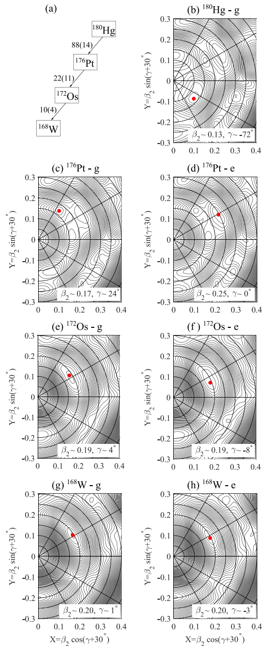
FIG. 12. (a) \alpha -decay chain from ^{180}\text{Hg} to ^{168}\text{W} . The relative HF value for the fine structure member to the first excited 2^+ state of each decay is shown to the left of each arrow, where the data are taken from Ref. [55] and the present measurement on ^{172}\text{Os} . Results of TRS calculations are shown for the ground-state configuration of ^{180}\text{Hg} [labeled (b)] and the ground-state and first excited 2^+ states of ^{176}\text{Pt} [(c) and (d), respectively], ^{172}\text{Os} [(e) and (f), respectively], and ^{168}\text{W} [(g) and (h), respectively]. The potential energy surfaces (PES) for the ground 0^+ states and the first excited 2^+ states were calculated at \hbar\omega = 0 and 0.15 MeV, respectively. The energy difference between contour lines in the PES is 100 keV. Minima in the PES are indicated by red dots with the corresponding deformation parameters shown in each panel. See text for details.
