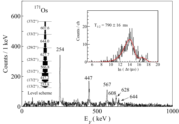
FIG. 5. Prompt RDT \gamma rays in JGII associated with the ^{171}\text{Os} ion implantation in the DSSDs followed by the \alpha decay of E_\alpha = 5306 keV within a maximum search time of 10 s in the same pixel. The inset shows the logarithmic time spectrum of the correlated recoil- \alpha events within a search time of 1 minute by gating on prompt 254 keV \gamma rays. The time distribution was fitted using a two-component Schmidt formula [22] as shown by the red line, and the component at higher \ln(\Delta t) values corresponds to the random-correlated events. A partial level scheme of the \nu i_{13/2} band in ^{171}\text{Os} reproduced from the NNDC database [17] is shown in the inset.
