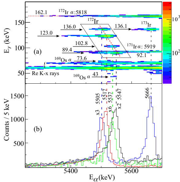
FIG. 9. (a) E_\alpha - E_\gamma coincidence spectrum with the time interval of 0 < \Delta t(\gamma-\alpha) < 300 ns. Each group is indicated with the corresponding energies. The parallelogram region indicates \alpha decays from the low-spin isomeric state of ^{172}\text{Ir} ; see text for details. (b) Projections on the E_\alpha axis of the events from the ^{172}\text{Ir} region of (a) by gating on the respective delayed \gamma rays. Relevant peaks are labeled with their corresponding E_\alpha values. The intensity scales for the three weaker spectra are adjusted for better visibility.
