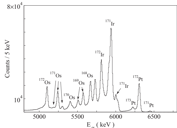
FIG. 1. Total \alpha -particle energy spectrum observed in the DSSDs. Assignments to the main \alpha decay lines are indicated.
