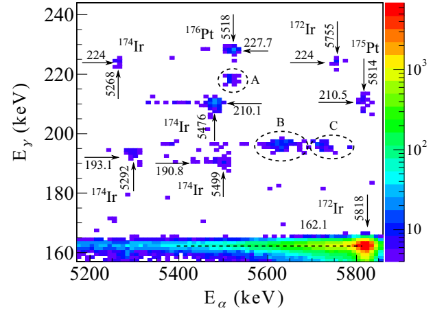
FIG. 10. E_\alpha - E_\gamma coincidence spectrum with the time interval of 0 < \Delta t(\gamma-\alpha) < 300 ns. Each group is annotated with the corresponding energies and the original mother nucleus, of which the ^{175}\text{Pt} and ^{176}\text{Pt} were due to the isotopic impurity in the target. The groups labeled with A, B, and C are due to decays that could not be firmly assigned to any nucleus.
