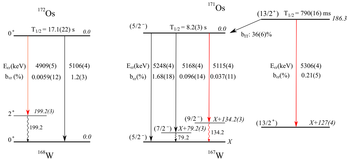
FIG. 7. Decay schemes of ^{172}\text{Os} and ^{171}\text{Os} deduced in this work apart from the branching ratio 1.68(18)% for the 5248 keV \alpha decay, taken from Ref. [17]. The energy of the (5/2^-) \alpha -decaying bandhead of ^{167}\text{W} is not established experimentally, and thus is tentatively indicated by X . The newly observed transitions are indicated in red. The determined half-life for each state from this work is shown above the state. See text and Table I for details.
