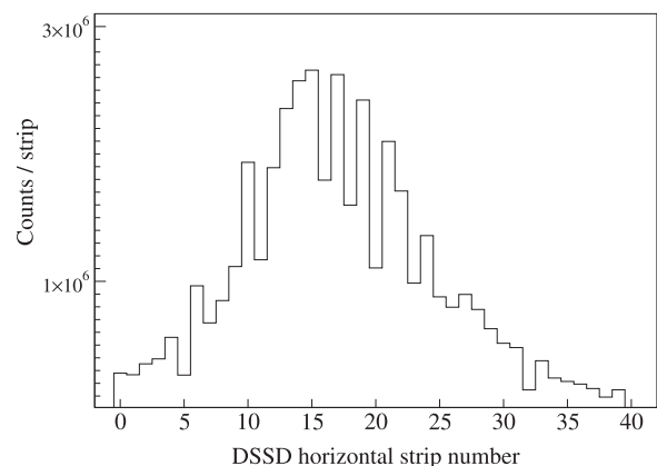
FIG. 2. The distribution of detected \alpha events in the horizontal strips of the DSSDs accumulated during the entire experiment.
