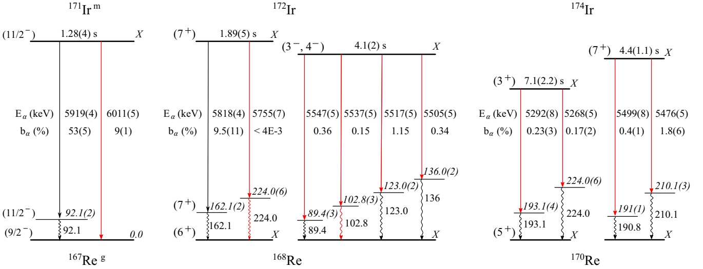
FIG. 11. Decay schemes of ^{171,172,174}\text{Ir} deduced in this work. Some levels are labeled with the symbol X indicating that their excitation energy relative to the ground state in the corresponding nuclide is unknown. The newly observed transitions are indicated in red. Half-lives determined from this work are shown above the corresponding state. See text and Table I for details.
