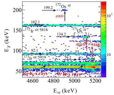
FIG. 4. E_\alpha - E_\gamma coincidence spectrum selected from events with the correlation time interval of < \Delta t(\gamma-\alpha) < 300 ns. All energies are given in keV. Each group is indicated with the corresponding energies and the arrows indicate the positions of the associated \alpha particles and \gamma rays; see details in the text.
