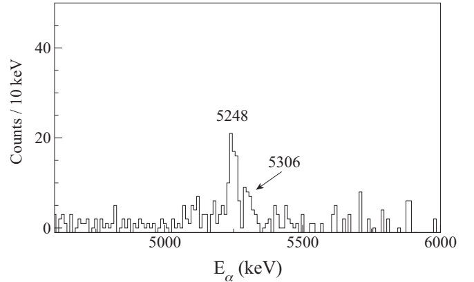
FIG. 6. Energy spectrum of \alpha decays in correlation with ^{171}\text{Os} recoil implantations and requiring additionally prompt \gamma - \gamma coincidences between the 254 keV \gamma -ray transition and either the 447, 567, or 628 keV \gamma -ray transitions of the \nu i_{13/2} band. Only the low-counting horizontal DSSD strips with the strip number larger than 28 or smaller than 6 were used for the analysis.
