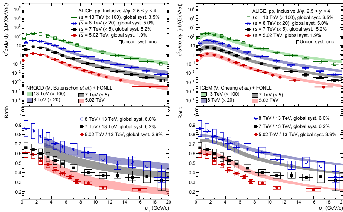
Fig. 9 Transverse momentum dependence of the inclusive J/\psi cross section, at forward y , measured in pp collisions at \sqrt{s} = 5.02 , 7 [12], 8 [13], and 13 TeV [9] (top panels), and ratio of the measurements at 5.02, 7, and 8 TeV to the 13 TeV data (bottom panels). The data are
