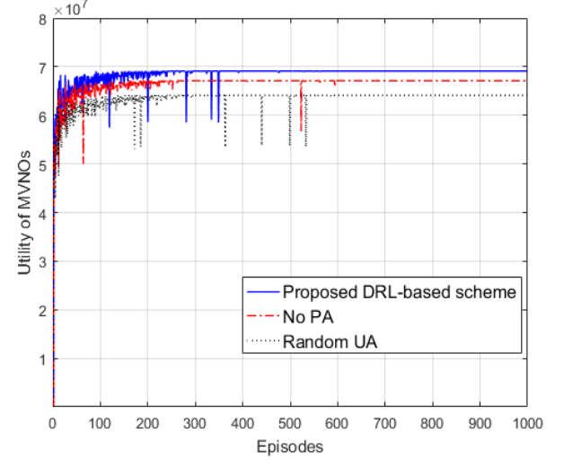
Fig. 4. Convergence performance of different DRL-based schemes.
