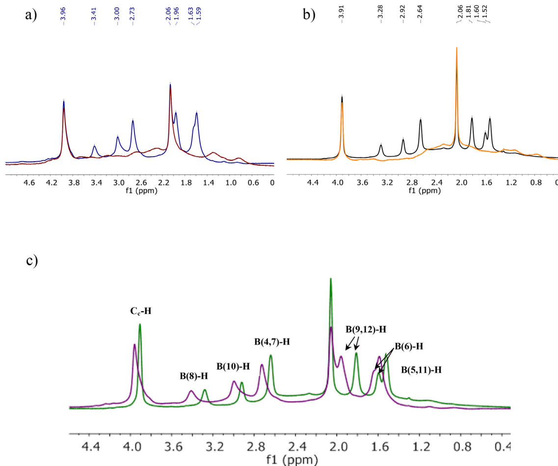
Fig. 1. a) Comparison between ^1\text{H} -NMR (red) and ^1\text{H}^{(11)\text{B}} -NMR (blue) for salt \text{Fe}[3,3'\text{-Co}(1,2\text{-C}_2\text{B}_9\text{H}_{11})_2]_2 . b) Comparison between ^1\text{H} -NMR (orange) and ^1\text{H}^{(11)\text{B}} -NMR (black) for compound \text{Fe}[3,3'\text{-Co}(1,2\text{-C}_2\text{B}_9\text{H}_{11})_2]_3 . c) ^1\text{H}^{(11)\text{B}} -NMR comparison between \text{Fe}[3,3'\text{-Co}(1,2\text{-C}_2\text{B}_9\text{H}_{11})_2]_2 (green) and \text{Fe}[3,3'\text{-Co}(1,2\text{-C}_2\text{B}_9\text{H}_{11})_2]_3 (purple).
