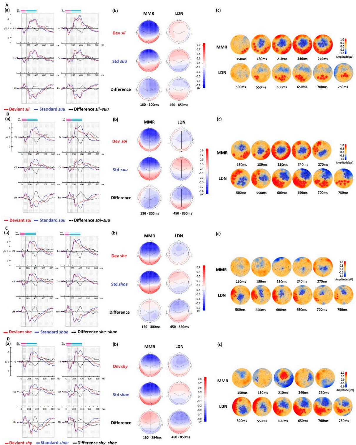
Figure 3. Average brain responses of the control group ( N = 86 ) to the native conditions (A) sii-suu and (B) sai-suu and to the foreign conditions (C) she-shoe and (D) shy-shoe . (a) ERP waveforms of the native language deviant in red, the standard in blue, and their difference wave deviant-standard in black. The windows of interest showing the MMR and the LDN components are highlighted in black boxes. (b) Corresponding means topographic maps over the MMR and LDN time windows. (c) The statistical cluster-based permutation test results showing significant differences between the responses to deviant and standard stimuli are indicated with stars. Blue and red colors indicate negative and positive amplitude values, respectively. The measuring unit is \mu\text{V} .
