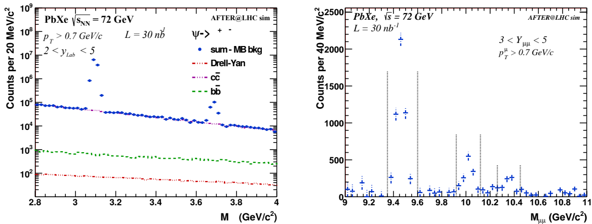
Figure 46: Di-muon invariant mass distribution in the J/\psi , \psi(2S) (Left) and \Upsilon(nS) (Right) regions, expected in PbXe FT collisions at \sqrt{s_{NN}} = 72 GeV, for an LHCb-like detector ( 2 < y_{lab} < 5 ). The combinatorial background is subtracted using like-sign pairs. No nuclear modification are assumed. The integrated luminosity of \int \mathcal{L} = 30\text{nb}^{-1} corresponds to one LHC-year of data-taking for ions (i.e. typically one month of data taking), with an LHCb-like detector equipped with a gaseous storage-cell of 1-m length. The maximum luminosity achieved has been limited such that no more than 15% of the Pb beam is removed by the interaction with the target. [Plots taken from [6]].
