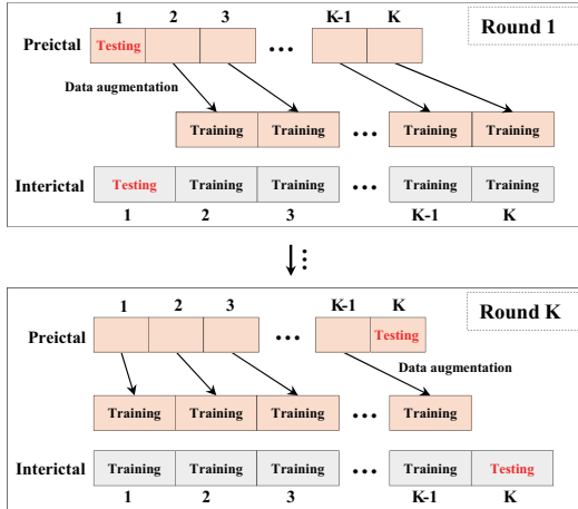
Fig. 3. The K-CV approach combined with the data augmentation technique is applied during model training.
