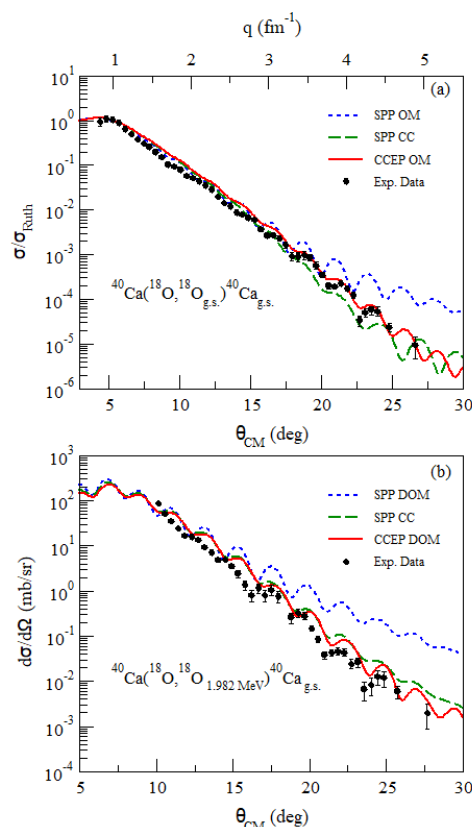
Figure 2. Panel (a): Cross section angular distribution of the ^{18}\text{O} + ^{40}\text{Ca} elastic scattering at 15 MeV/u in terms of its ratio to the Rutherford cross section. Panel (b): Angular distribution of the inelastic channel ^{40}\text{Ca}(^{18}\text{O}, ^{18}\text{O}_{1.982})^{40}\text{Ca}_{\text{g.s.}} . In both plots, the blue dotted line shows the optical model (OM) and distorted wave Born approximation (DOM) calculations with the SPP, the green dashed line shows the CC calculations with SPP, and the red solid line shows the OM and DOM calculations with CCEP. From Ref. [9].
