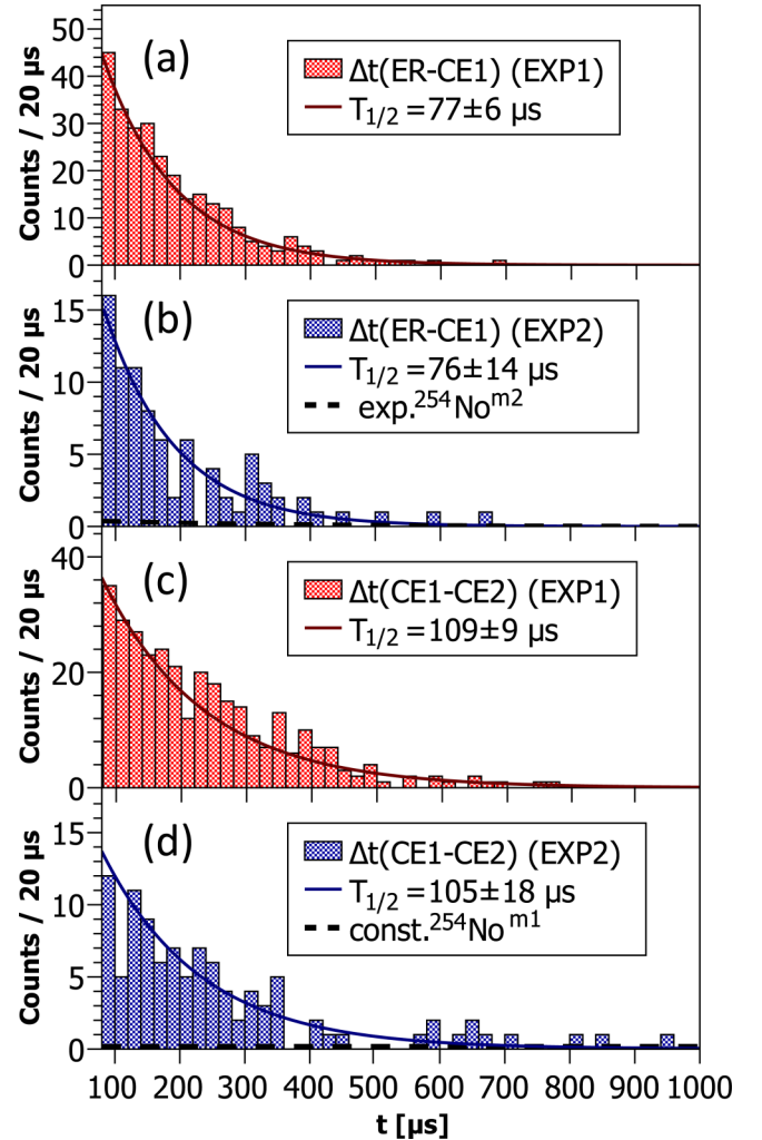
FIG. 3. Time-difference distributions in the range 80–1000 \mu\text{s} between implantation of ER and registration of CE1 in (a) Exp1 (red), (b) Exp2 (blue), or between registration of CE1 and CE2 in (c) Exp1 (red), (d) Exp2 (blue). Solid red and blue lines represent the fits of the data with exponential functions. Dashed black lines denote contributions from ^{254}\text{No}^{m2} in (b) and ^{254}\text{No}^{m1} in (d), respectively.
