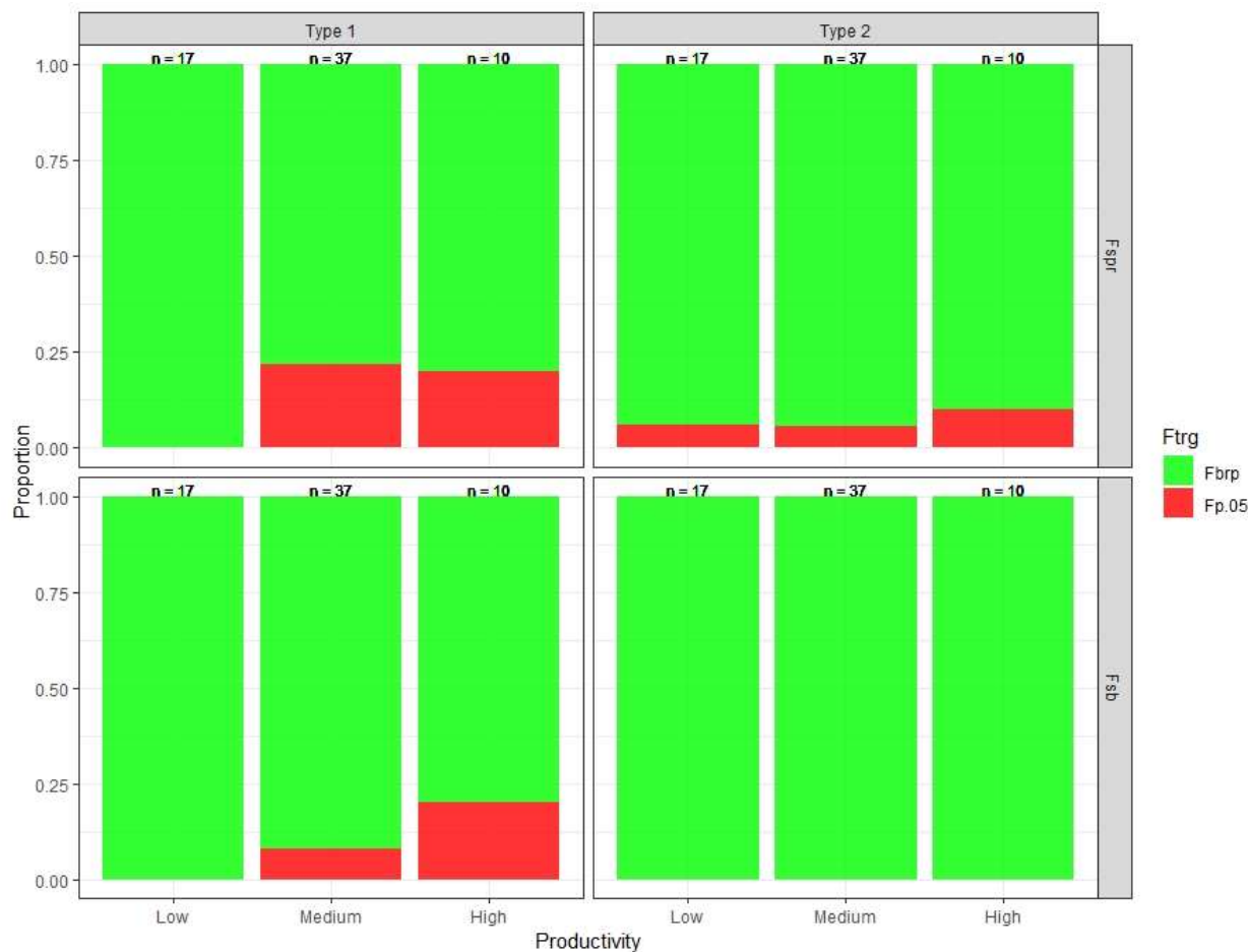
Figure 9: Proportion of stocks triggering F_{p.05} for the different category of productivity when using F_{SPR\%} or F_{B\%}
