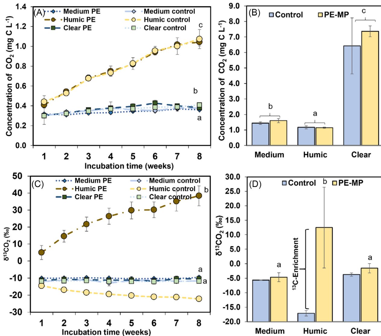
FIGURE 2 The concentration of CO 2 and respiration of 13 C-PE into CO 2 . (A) The concentration of carbon dioxide (respiration) in the headspace and (B) the water during the 8-week incubation of polyethylene (PE, n = 3) and controls (no-PE, n = 2) in the artificial medium (medium), clear eutrophic (clear) and humic mesotrophic (humic) lake water. The development of δ 13 C value of carbon dioxide in the (C) headspace and (D) water during the 8-week incubation in the artificial freshwater medium (medium), humic-lake water (humic), and clear-lake water eutrophic (clear). Letters in A and C cite the statistical difference between waters (PE treatments), c > b > a , p < 0.05. Letters in B and D cite the statistical differences between waters (PE + control), which explained most of the variation among treatments, c > b > a , p < 0.05.
