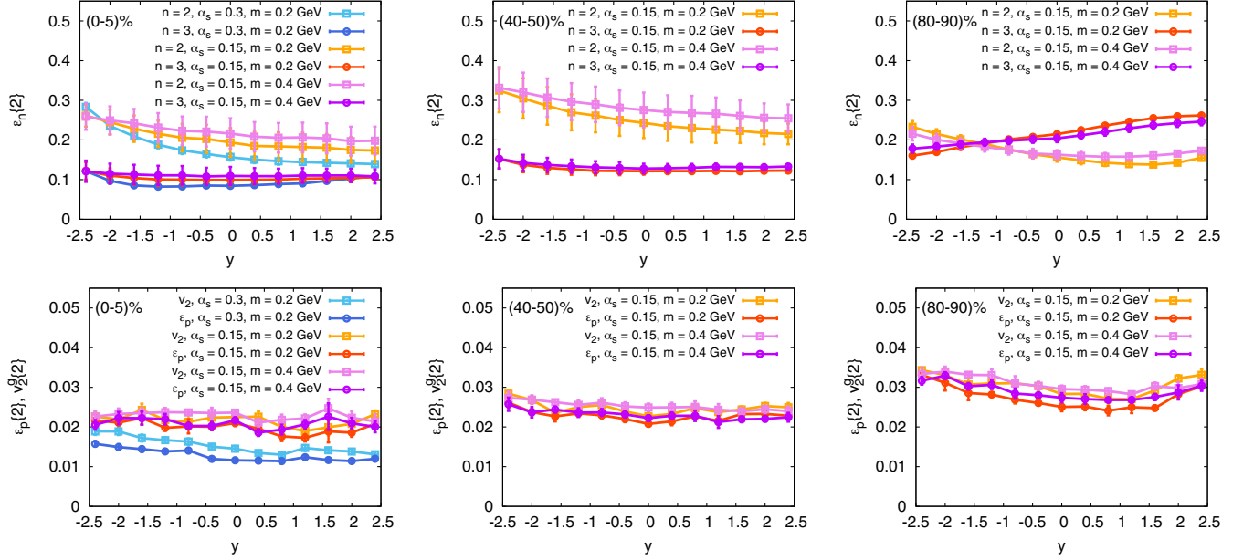
FIG. 6. Geometric eccentricities \epsilon_n\{2\} = \sqrt{\langle |\epsilon_n(y)|^2 \rangle} (top row) and initial momentum anisotropies \epsilon_p\{2\} = \sqrt{\langle |\epsilon_p(y)|^2 \rangle} together with azimuthal anisotropy v_2^g\{2\} = \sqrt{\langle |v_2^g(y)|^2 \rangle} (bottom row) for different centrality classes 0%–5% (left panels), 40%–50% (center panels), and 80%–90% (right panels) as a function of rapidity.
