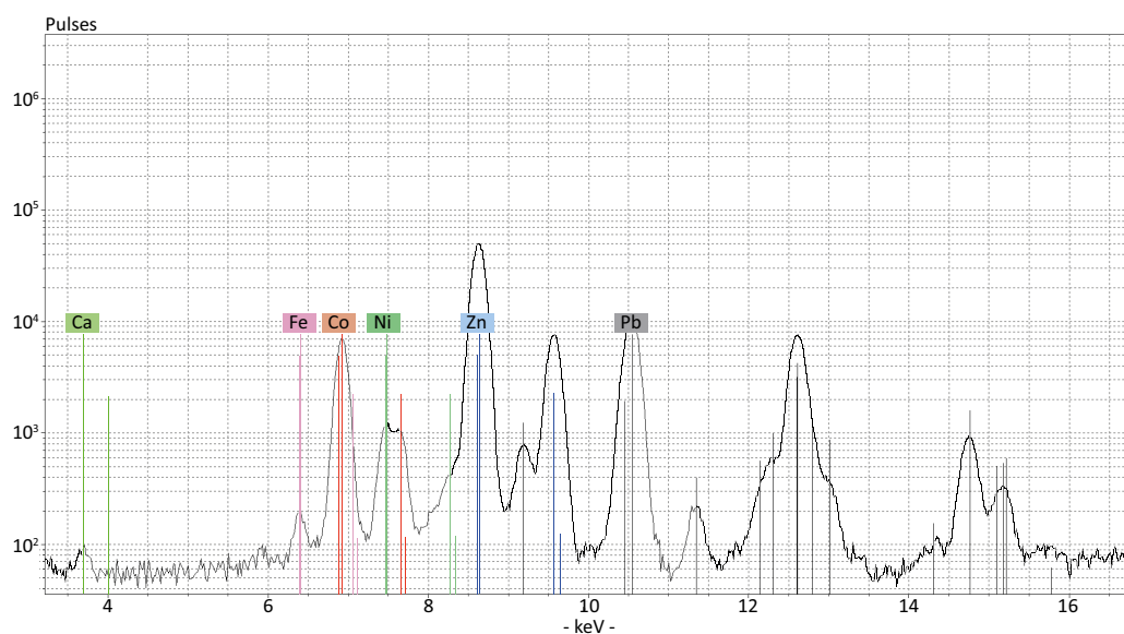
Spectrum 1. EDXRF spectrum measured from the blue area of Akseli Gallen-Kallela's painting Portrait of Carl Gustaf Mannerheim, sketch . Private collection
