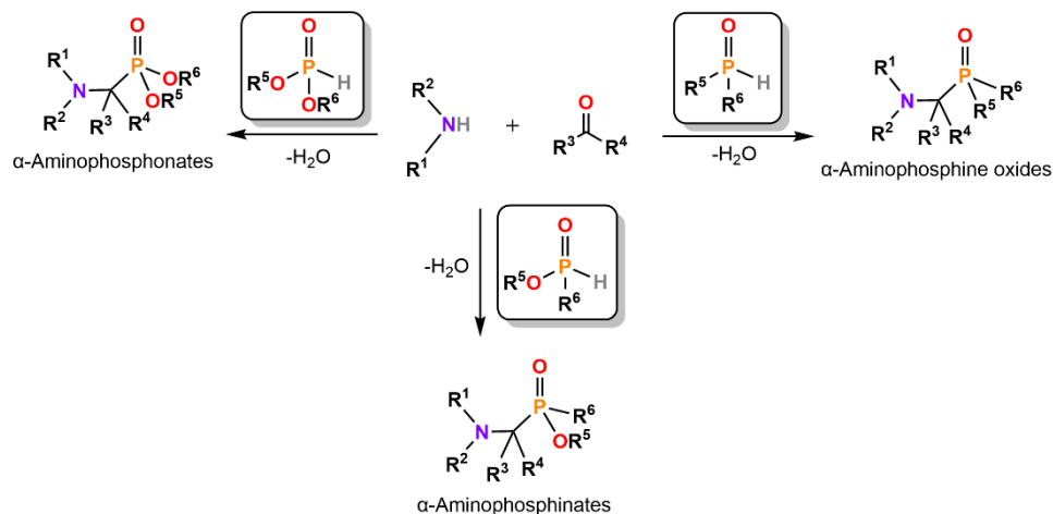
Scheme 3. The general route for Kabachnik–Fields reaction for α-aminophosphonates, -phosphinates, and -phosphine oxides. Substituents R 1 –R 6 can be either H, alkyl, or aryl substituents.
