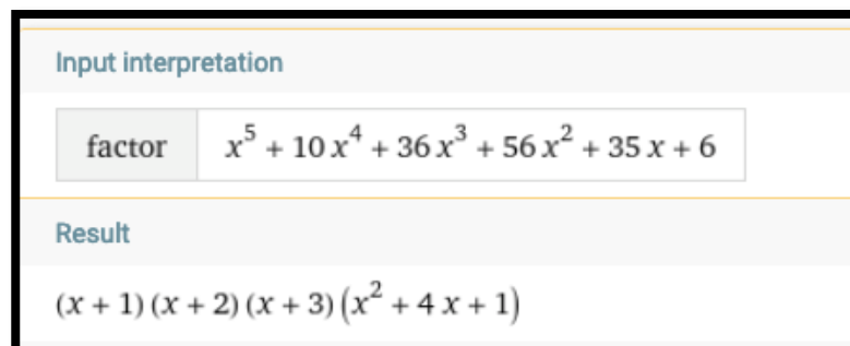
Figure 3. Factoring a Fibonacci-like polynomial.
