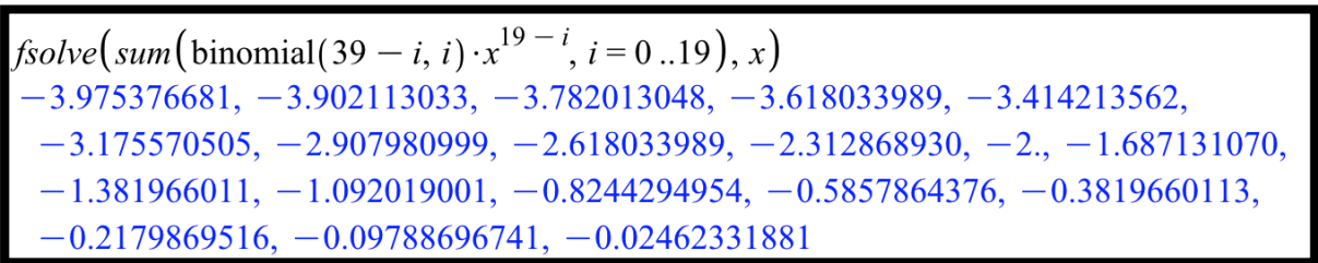
Figure 5. The roots of the equation P_{38}(x) = 0 .
