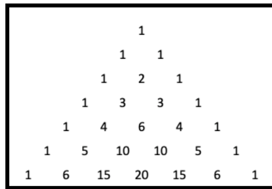
Figure 1. Pascal's triangle.
