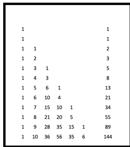
Figure 2. Rearranged Pascal's triangle and Fibonacci numbers.
