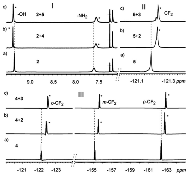
Fig. 5 I: ^1\text{H} NMR spectra (in \text{CDCl}_3 at 303 K) of: (a) 2 (30 mM), (b) a 1 : 4 mixture of 2 and 4, and (c) a 1 : 4 mixture of 2 and 5. II: ^{19}\text{F} NMR of: (a) 5 (30 mM), (b) a 4 : 1 mixture of 5 and 2, and (c) a 4 : 1 mixture of 5 and 3. III: ^{19}\text{F} NMR spectra of: (a) 4 (30 mM), (b) a 4 : 1 mixture of 4 and 2, (c) a 4 : 1 mixture of 4 and 3.
