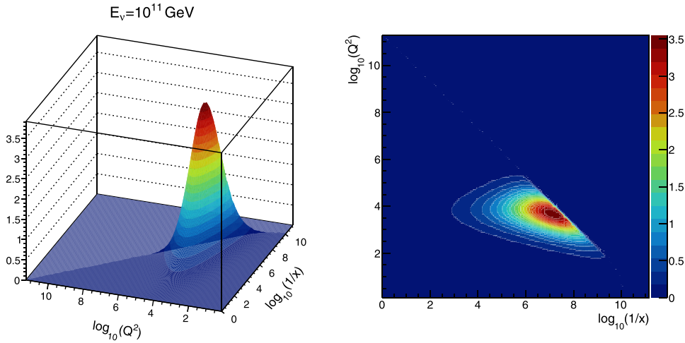
Figure 47. Differential CC neutrino cross-section 10^5 \times xQ^2 d\sigma^{CC}/dx dQ^2 (nb) as a function of Q^2 and x for a fixed neutrino energy of E_\nu = 10^{11} GeV. Left: surface plot; right: contour plot.
