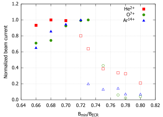
FIG. 15. Behavior of \text{He}^{2+} , \text{O}^{7+} , and \text{Ar}^{14+} beam currents with increasing B_{\min}/B_{\text{ECR}} -ratio, measured with the JYFL 14 GHz ECRIS. The solid and open symbols represent stable and unstable plasma conditions, respectively. Reproduced from Tarvainen et al. , Rev. Sci. Instrum. 87 , 02A701 (2016) with the permission of AIP Publishing.
