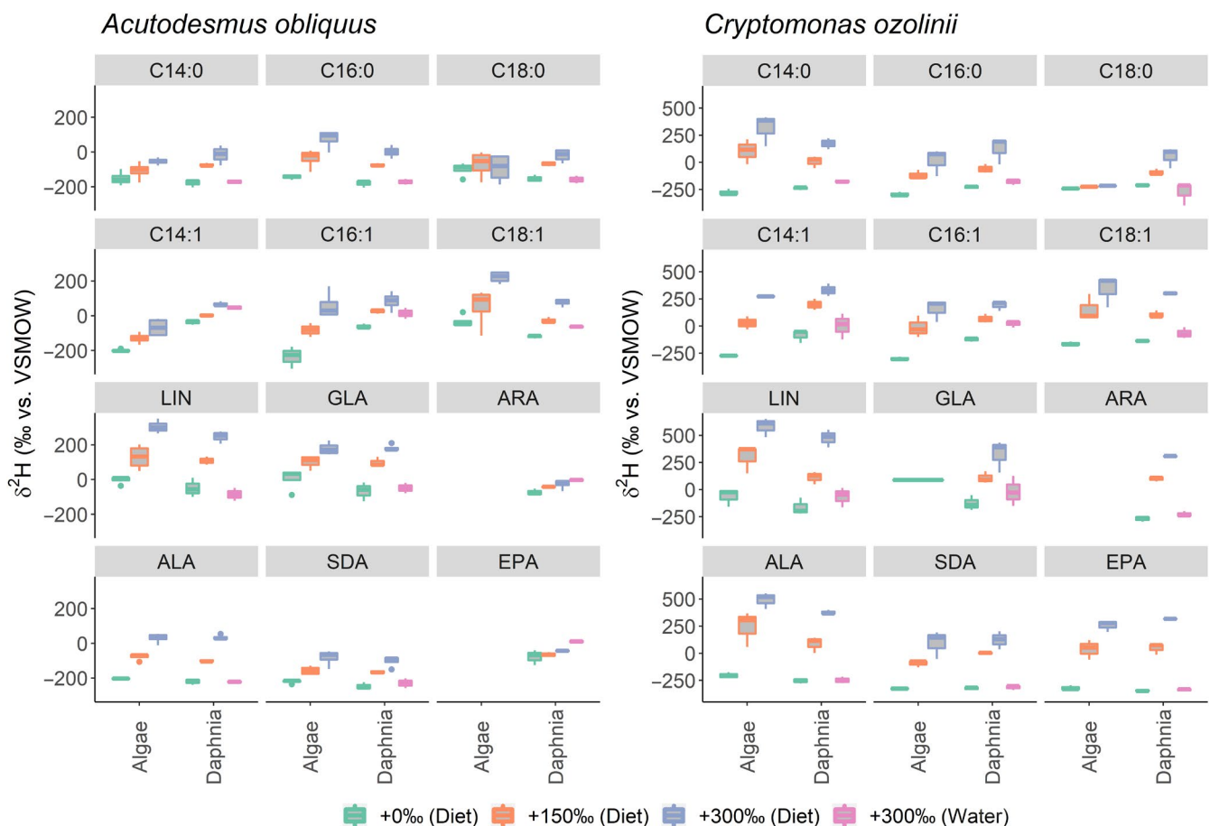
FIGURE 2 Compound-specific deuterium allocation into fatty acids of Daphnia via diet (green, orange and blue) or environmental water (purple). MUFA experienced significant changes in \delta^2\text{H} values, as well as a significant enrichment in deuterium when Daphnia were raised in ^2\text{H}_2\text{O} , indicating FA synthesis. Strict dietary controlled allocation of fatty acids can be seen for LIN and ALA. Deuterium enrichment in ARA and EPA can be seen in Daphnia when raised in deuterium-enriched environmental water with poor diet quality ( Acutodesmus obliquus ) but not with high diet quality ( Cryptomonas ozolinii ) in which case EPA is also strictly dietary controlled
