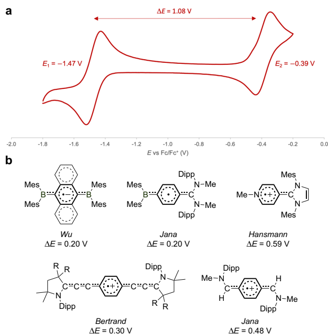
Fig. 3 Electrochemical studies. a Cyclic voltammogram of 1 ( [^{10}Bu_4N][PF_6] in CH_2Cl_2 at 100 mV s^{-1} ). b Redox ranges associated with related structurally characterized radicals (Hansmann et al. reported in ref. 12 that a related radical cation [(MeCMesN)_2C(C_5H_4N)Trip]^{\bullet+} has redox range \Delta E = 0.72 V, but this species has not been structurally characterized).
