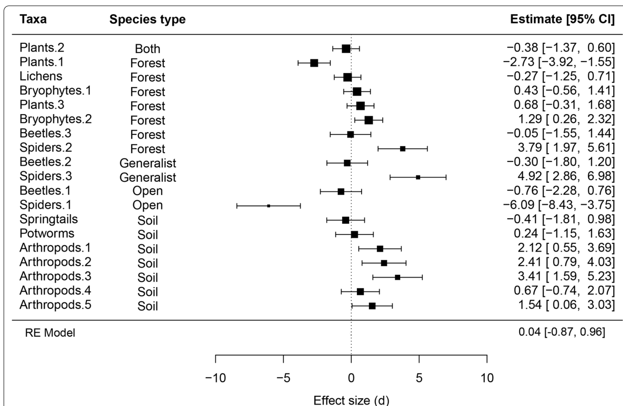
Fig. 12 Forest plot of effect sizes for individual abundance (mean standardized difference between uneven-aged and retention forest). Effect sizes to the right of zero mean uneven-aged forest has more individuals than retention forest. Different habitat specialisms of the taxa are given. The category 'both' includes both open habitat and forest dependent species. Numbers after the taxa denote different studies. The error bars represent 95% confidence intervals. Effect size below the bottom line on the right is the overall effect with 95% confidence intervals
